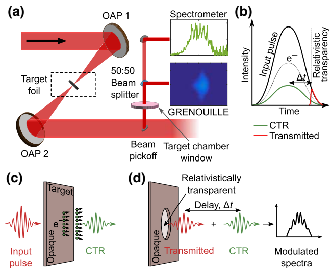
FIG. 1. (a) Schematic of the experiment showing the laser-focusing geometry and diagnostic channel. The drive laser pulse is focused using off-axis parabola OAP 1 and the light collected at the target rear, using OAP 2, is directed for simultaneous measurement using a GRENOUILLE and an optical spectrometer. (b) Schematic illustrating the timing of the CTR generation and transmitted part of the laser pulse, where the temporal separation ( \Delta t ) relates to the onset time of RSIT relative to the peak of the laser pulse interacting and fast electron generation. (c,d) Schematic of the laser-plasma interaction before, (c), and after, (d), RSIT, resulting in a generated pulse of CTR light and the transmitted laser pulse, with a temporal delay defined by the onset time for RSIT.
