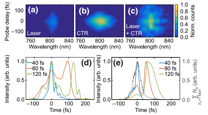
FIG. 2. FROG measurements of the transmitted and/or generated light for (a) no target, (b) d = 37 nm, (c) d = 30 nm; all for \tau_L = 40 fs. (d) Temporal-intensity profile of light measured at the target rear side extracted from example GRENOUILLE measurements for d = 30 nm, for three given durations of the drive laser pulse. (e) Corresponding results from three-dimensional (3D) EPOCH PIC simulations, including a plot of the total number of electrons (with energy > 1 MeV) as a function of time, for the 80-fs pulse-duration case.
