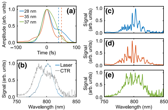
FIG. 4. (a) Temporal-intensity profile extracted from GRENOUILLE measurements for three given target thicknesses, for fixed drive laser pulse duration \tau_L = 40 fs. (b) Representative measurements of the input laser spectrum and the generated CTR spectrum. (c)–(e) Spectral measurements for (c) d = 28 nm, (d) d = 35 nm, and (e) d = 37 nm targets.
