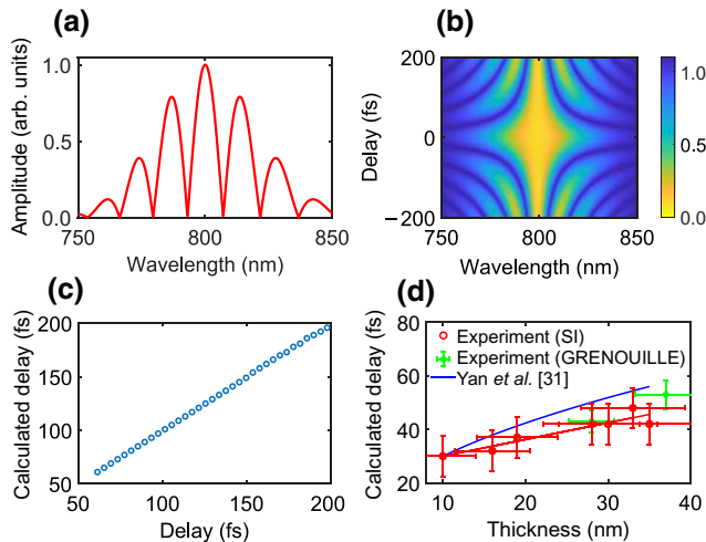
FIG. 5. (a) Model spectrum for the superposition of two identical pulses with \tau_L = 40 fs and \Delta t = 150 fs, illustrating spectral fringes. (b) Spectral fringe pattern as a function of \Delta t , from -200 to 200 fs. (c) Calculated delay from a Fourier transform of the spectrum, as a function of the input delay. (d) Delay determined from a Fourier transform of the measured spectra in the experiment, as a function of target thickness (red points) and the points measured using the GRENOUILLE (for comparison), for \tau_L = 40 fs. Calculated time for the target to become transparent to the laser using the plasma-expansion model reported in Yan et al. [31] (blue).
