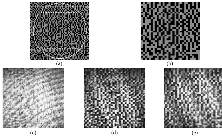
Fig. 8. Experimental results. (a) Signal pattern \phi(x, y) . Solid and dashed lines enclose the area to be recorded and the area used for SNR calculation, respectively. Dark pixels represent \pi/2 pixels, whereas brighter pixels represent 0 pixels. (b) Enlarged view of the region for SNR calculation [area enclosed by dashed line in (a)]. (c) Directly captured writing beam, i.e., intensity distribution of \phi^w(x, y) . (d) Output intensity pattern in storage-type SRH. (e) Output intensity pattern in PIC-type SRH.
