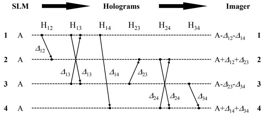
Fig. 4. Conceptual diagram of energy interchanges between four pixels. In this example, the intensities of pixels 1 and 3 are lower than those of pixels 2 and 4 at the output.
