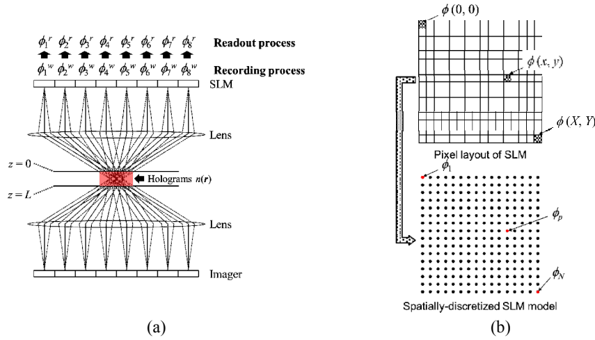
Fig. 2. Models for theoretical description of SRH principle. (a) Overview of the model. Light from the SLM pixels is converted to plane waves by a lens. These plane waves interfere with each other, and holograms are generated. (b) Layout of SLM. In the theoretical description, the pixels of the SLM are regarded as a set of many point sources.
