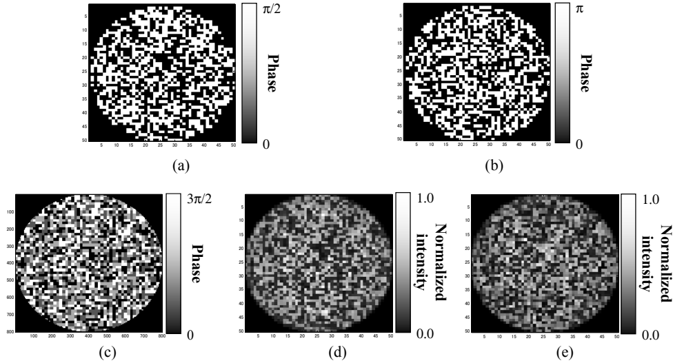
Fig. 6. Simulation results. (a) Signal pattern \phi(x, y) . This pattern is used as the signal to be recorded in storage-type SRH and as the target to be detected in PIC-type SRH. (b) Additional pattern \phi^{ad}(x, y) . This pattern is recorded in PIC-type SRH. (c) Writing pattern \phi^v(x, y) = \phi(x, y) + \phi^{ad}(x, y) for storage-type SRH. Readout pattern for PIC-type SRH. (d) Normalized output intensity pattern of storage-type SRH. (e) Normalized output intensity pattern of PIC-type SRH.
