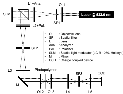
Fig. 7. Experimental setup. Light source was a diode-pumped solid-state laser with a wavelength of 532.0 nm. Focal lengths of L1, L2, L3, L4, and L5 are 150, 200, 200, 100, and 100 mm, respectively.
