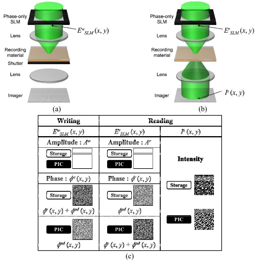
Fig. 1. Conceptual diagram of self-referential holography. (a) Optical geometry for recording. The writing beam with a complex amplitude of E^w_{SLM}(x, y) is focused by an objective lens, and holograms are generated by self-interference between recording pixels. (b) The readout beam with a complex amplitude of E^r_{SLM}(x, y) is focused by an objective lens. The uniform readout intensity is changed to the signal intensity pattern F^s(x, y) via the energy interchanges in the holograms. (c) Complex amplitudes of writing and readout beams. The patterns \phi^w(x, y) and \phi^r(x, y) are added to the writing and readout beams, respectively. If \phi^w(x, y) - \phi^r(x, y) \equiv \pm \phi(x, y) , the intensity pattern that corresponds to the distribution of \pm \phi(x, y) can be observed.
