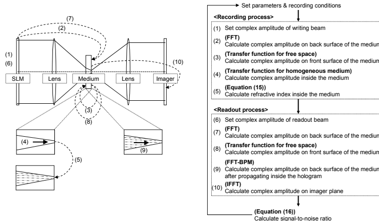
Fig. 5. Models and flows in FFT-BPM-based simulations.
