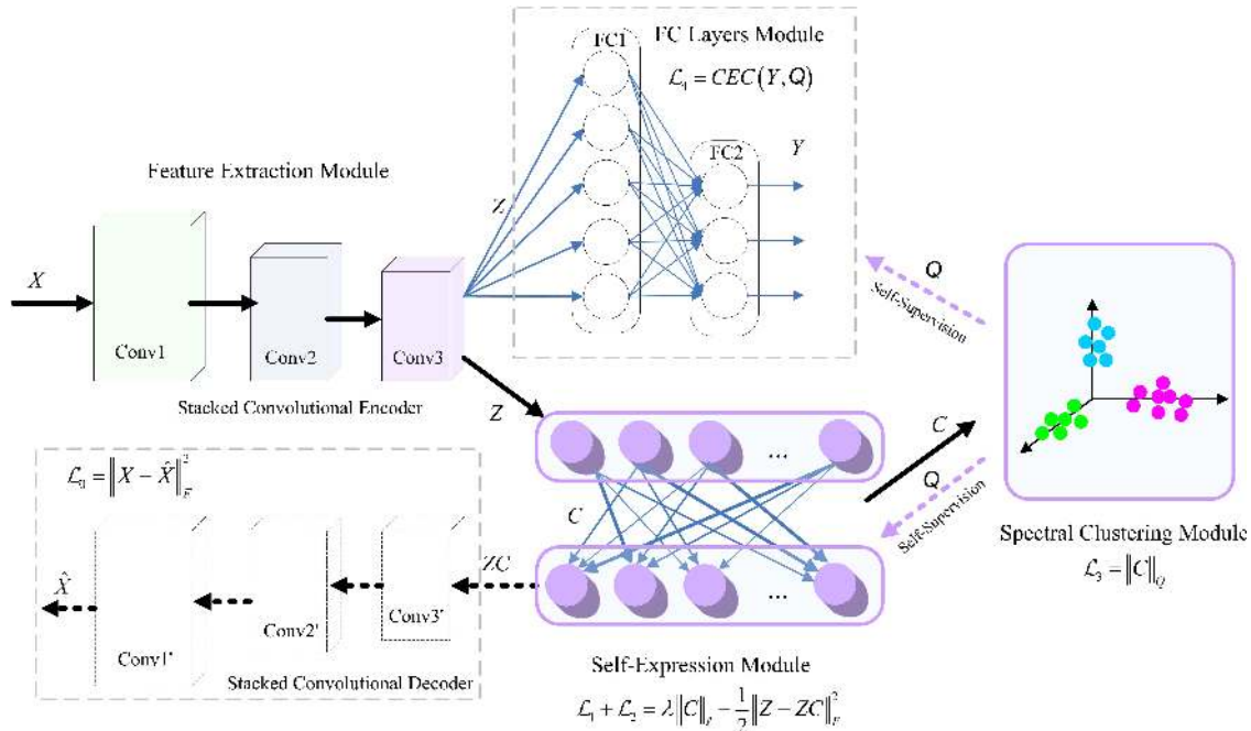
Figure 1. Architecture of the proposed Self-Supervised Convolutional Subspace Clustering Network (S 2 ConvSCN). It consists of mainly five modules: a) stacked convolutional encoder module, which is used to extract convolutional features; b) stacked convolutional decoder module, which is used with the encoder module to initialize the convolutional module; c) self-expression module, which is used to learn the self-expressive coefficient matrix and also takes the self-supervision information from the result of spectral clustering to refine the self-expressive coefficients matrix; d) FC-layers based self-supervision module, which builds a self-supervision path back to the stacked convolutional encoder module; e) spectral clustering module, which provides self-supervision information to guide the self-expressive model and FC-layers module. The modules with solid line box are the backbone components; whereas the modules in dashed box are the auxiliary components to facilitate the training of the whole network.
