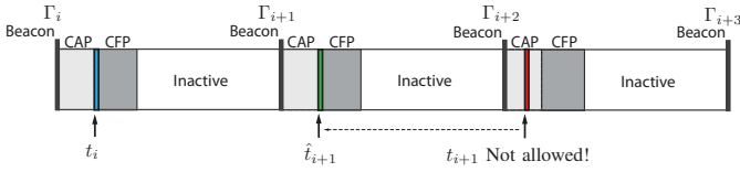
Fig. 2: EDF Scheduling over WSANs. Here we describe the scheduling of one of the nodes in the network using the self-triggered control scheme. The required triggering time t_{i+1} is not allowed since it does not occur during a CFP. An adjustment of this time to \hat{t}_{i+1} is made in order to allocate t_{i+1} inside a GTS and guarantee (6) under EDF scheduling.
