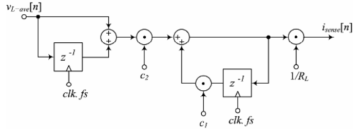
Fig.5. The architecture of the tunable IIR filter used in the current estimator.
