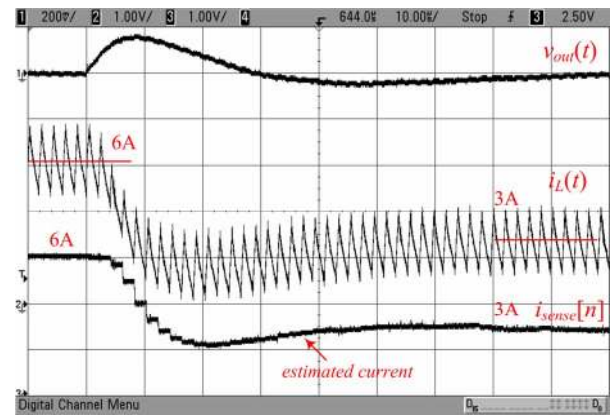
Fig.12. The estimated current during heavy-to-light load step between 6A and 3A– Ch1: Output converter voltage (200mV/div); Ch2: actual inductor current i_L(t) - 2 A/V; Ch3: estimated average current i_L[n] - 2 A/V; Time scale is 10 \mu s/div.
