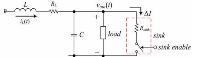
Fig. 3. Test current sink used for the filter calibration.
