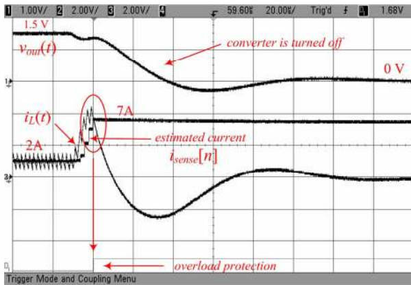
Fig.13. The overload protection implemented with the current estimator– Ch1: Output converter voltage (1V/div); Ch2: actual inductor current i_L(t) – 2 A/V; Ch3: estimated average current i_L[n] – 2 A/V; Time scale is 20 \mu s/div.
