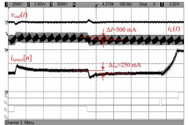
Fig.9. The calibration procedure using a 0.5A current sink – Ch1: Output converter voltage (200mV/div); Ch2: actual inductor current i_L(t) - 2 A/V; Ch3: estimated average current i_L[n] - 2 A/V; D0-D3- control signals; Time scale is 100 \mu s/div.
