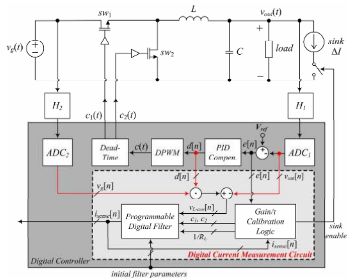
Fig. 1. A digitally-controlled buck converter with the self-tuning current estimator.
