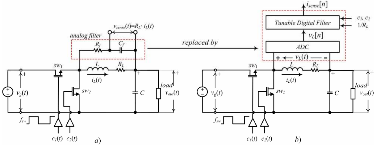
Fig. 2. Current sensing techniques: a) conventional analog implementation b) implementation with a self-tuning digital filter.
