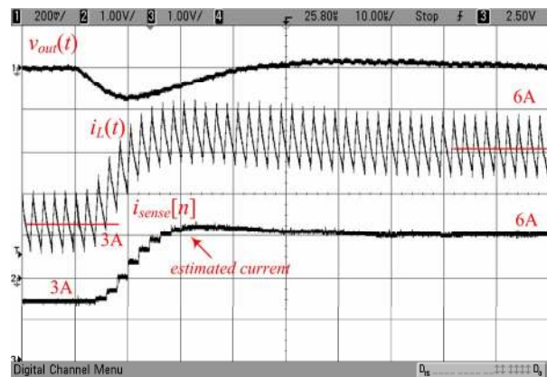
Fig. 11. The estimated current during light-to-heavy load step between 3A and 6A– Ch1: Output converter voltage (200mV/div); Ch2: actual inductor current i_L(t) - 2 A/V; Ch3: estimated average current i_L[n] - 2 A/V; Time scale is 10 \mu s/div.
