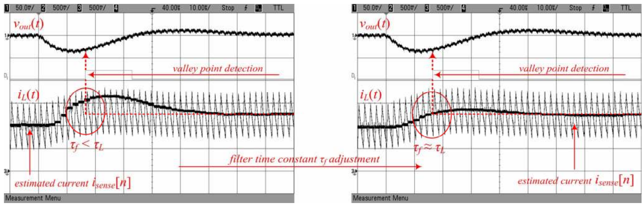
Fig.10. The estimator IIR filter time constant \tau_f is tuned (left) iteratively to match the inductor time constant \tau_L (right): Output converter voltage (50mV/div); Ch2: actual inductor current i_L(t) - 2 A/V; Ch3: estimated average current i_L[n] - 2 A/V; Time scale is 10 \mu s/div.
