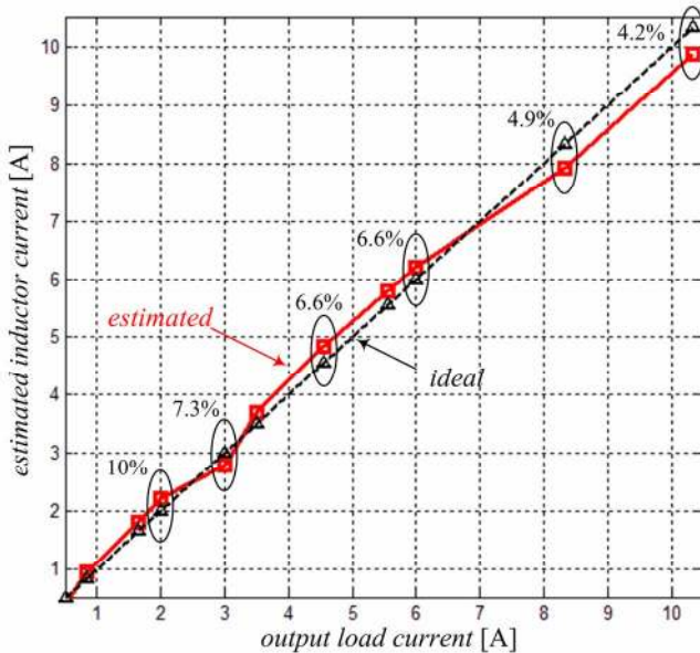
Fig. 14. Estimated inductor current versus the output load current
