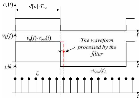
Fig. 4. Signals of a system implemented with an over-sampling ADC.
