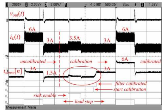
Fig.8. The system operation – Ch1: Output converter voltage (200mV/div); Ch2: actual inductor current i_L(t) - 2 A/V; Ch3: estimated average current i_L[n] - 2 A/V; D0-D3- control signals; Time scale is 500 \mu s/div.
