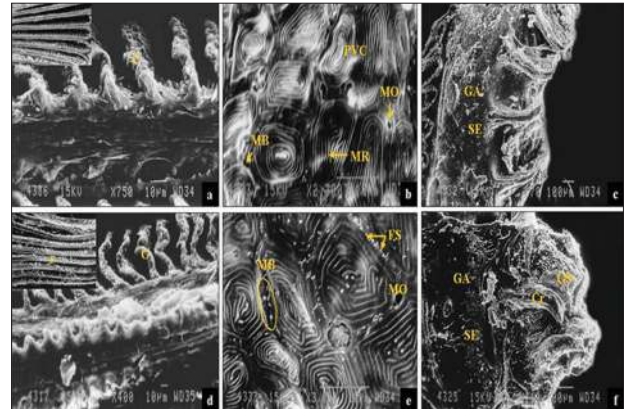
Fig. 2. Scanning electron micrographs of gills of Ctenopharyngodon idella on exposure to chlorpyrifos for 30 days at 1.44 µg/L CPF (a-c) and 2.41 µg/L CPF (d-f) showing marked damage of lamellar structure in form of fusion, curling and necrosis (a, d), marginal breakage (MB) and swollen microridges (MR) of pavement cells (b), severe marginal breakage and presence of filamentous strands on the border of PVC (e), presence of globular structures and cracks near gill raker (f). C – curling, Cr – cracks, D – degeneration, F – fusion, FS – filamentous strands, GA – gill arch, GR – gill raker, GS – globular structure, MB – marginal breakage, MO – mucosal opening, MR – microridges, PVC – pavement cells, SE – sloughed-off epithelium.
