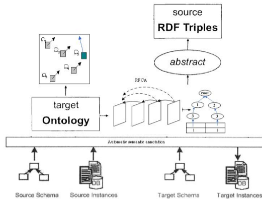
Figure 2. Semantic Annotation based on Rough Concept Lattice Model
