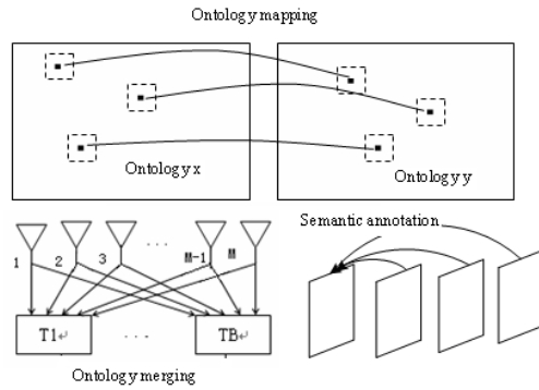
Figure 1. Semantic Annotation based on Ontology Mapping and Merging Structure Diagram
