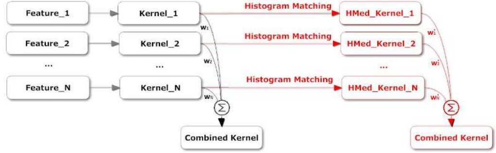
FIGURE 3.1: Typical feature combination methods always represent features into their kernel forms. These kernels are then combined. Traditionally, the kernels are combined directly through one of the methods in (3.2) or (3.3). In this chapter, we proposed to add a histogram matching module before these kernels are combined by one of the methods in (3.2) or (3.3).
