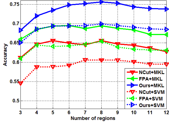
FIGURE 4.5: Global pixel accuracy on MSRC21
