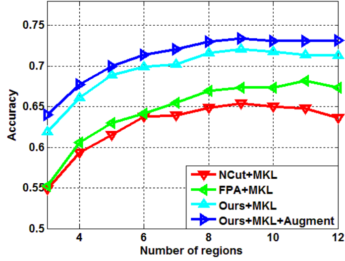
FIGURE 4.7: Semantic class accuracy on Stanford background dataset. 'Ours+Augment' represents results obtained by augmenting the training set.
