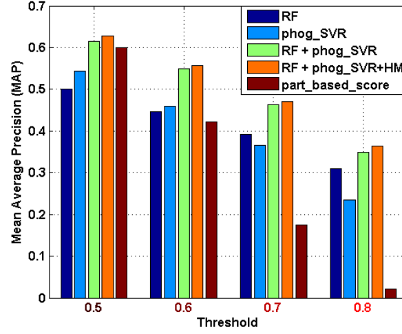
FIGURE 5.10: MAP value at different thresholds.
