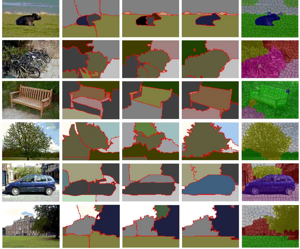
FIGURE 4.4: Some examples of the results of three segmentation methods. Each image is segmented into a predefined 7 regions. From left column to right column: original image; results generated by NCuts, Full Pairwise Affinity (FPA) [102], and our full model. The results of a typical semantic segmentation algorithm [101] is also shown in the last column.
