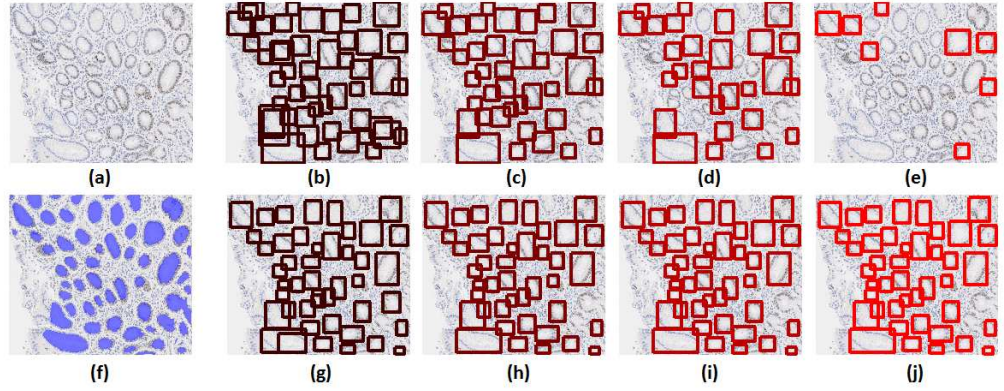
FIGURE 5.11: (a) The original microscopic image. (f) The ground truth image of glands. (b)-(e) The detection results obtained by [61] with threshold varies from 0.5 to 0.8 (g)-(j) The results obtained by by our model. As the threshold increases, the bounding boxes have to be more accurate. As the accuracy requirements increases (higher threshold), the detection result of [61] dropped significantly.
