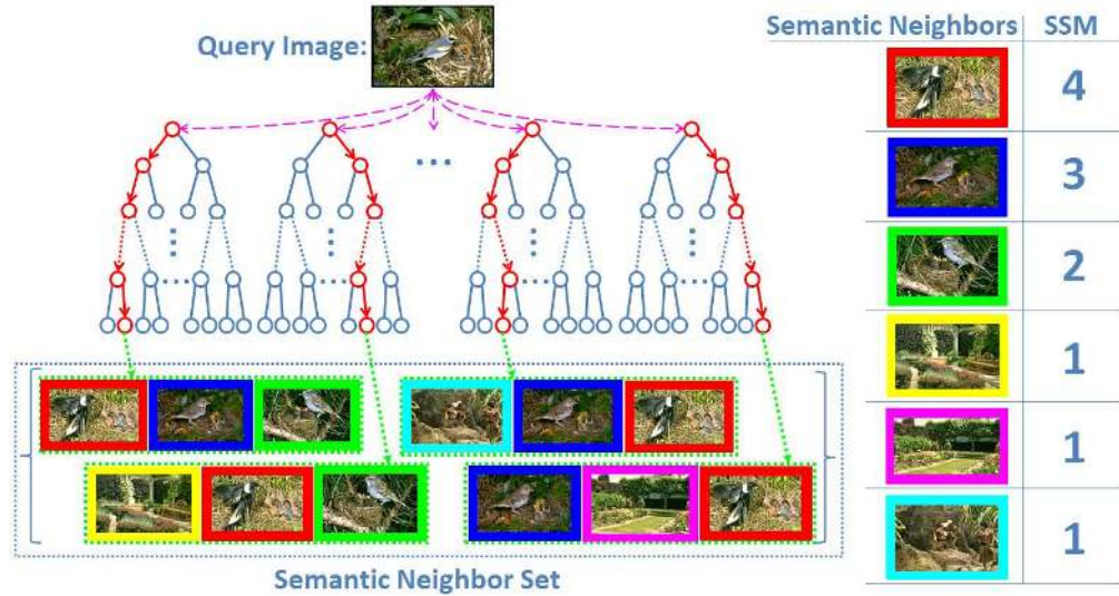
FIGURE 6.2: An example showing the concepts of semantic neighbor set and semantic neighbors. A query image passes through all random trees. The training images stored at the leaf nodes on which the query image falls into form the semantic neighbor set. Based on this, the semantic similarity measure (SSM) between the query and a particular training image is calculated as the number of times that the particular training image appears in the semantic neighbor set. A larger SSM indicates higher similarity.
