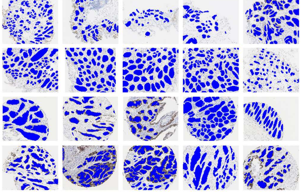
FIGURE 5.7: Nott-Gland dataset.
