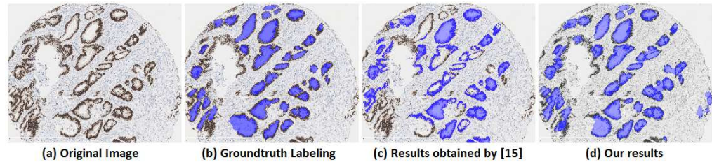
FIGURE 5.12: Segmentation results.
