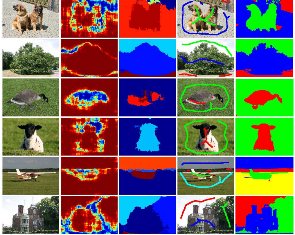
FIGURE 4.9: From left to right: original image; outputs from the semantic segmentation algorithm; the predicted semantic class; automatically generated tokens; segmentation results generated by [114] based on the tokens.
