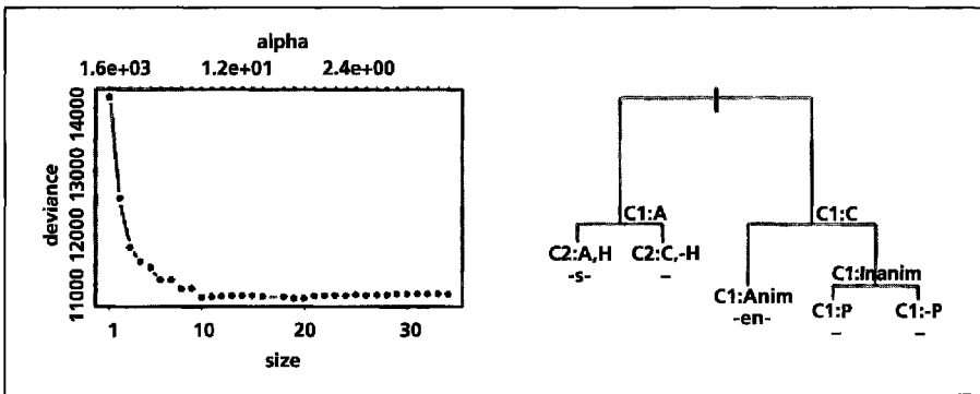
Figure 1: analysis of the semantic classes of the constituents of 6949 Dutch compounds as predictor variable and linker (-en-, -s-, and — in the case of a zero realization) as the response variable; left panel: plot of deviance versus tree size for sequences of subtrees; right panel: pruned classification tree; C1 = first constituent; C2 = second constituent; A = abstract; C = concrete; H = human being; Anim = animate; Inanim = inanimate; P = plant.
