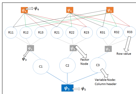
Fig. 5: This factor graph is a parameterized Markov network wherein the square nodes represent factor nodes.
