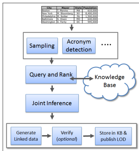
Fig. 3: Our extensible and domain independent framework relies on a joint inference module to generate a representation of the the meaning of the table as a whole.
