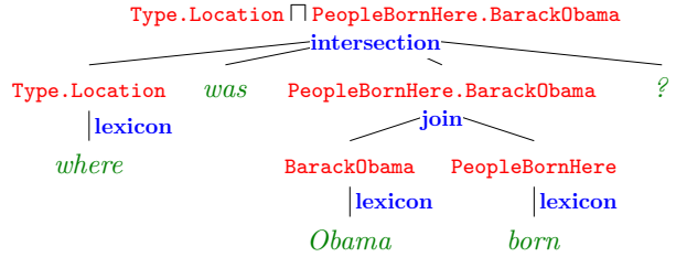
Figure 2: An example of a derivation d of the utterance “ Where was Obama born? ” and its sub-derivations, each labeled with composition rule (in blue) and logical form (in red). The derivation d skips the words “ was ” and “ ? ”.
