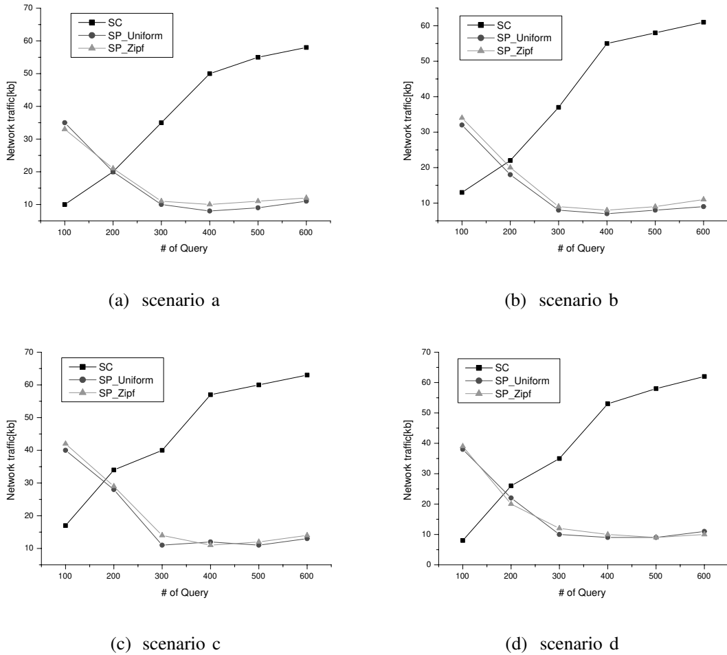
Fig. 13. Comparison of network traffic.
