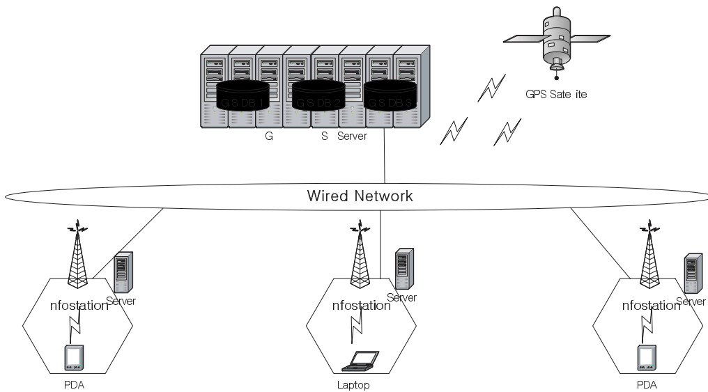
Fig. 2. Infostation architecture.
