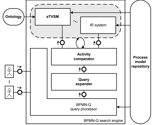
Figure 4. BPMN-Q search engine architecture
