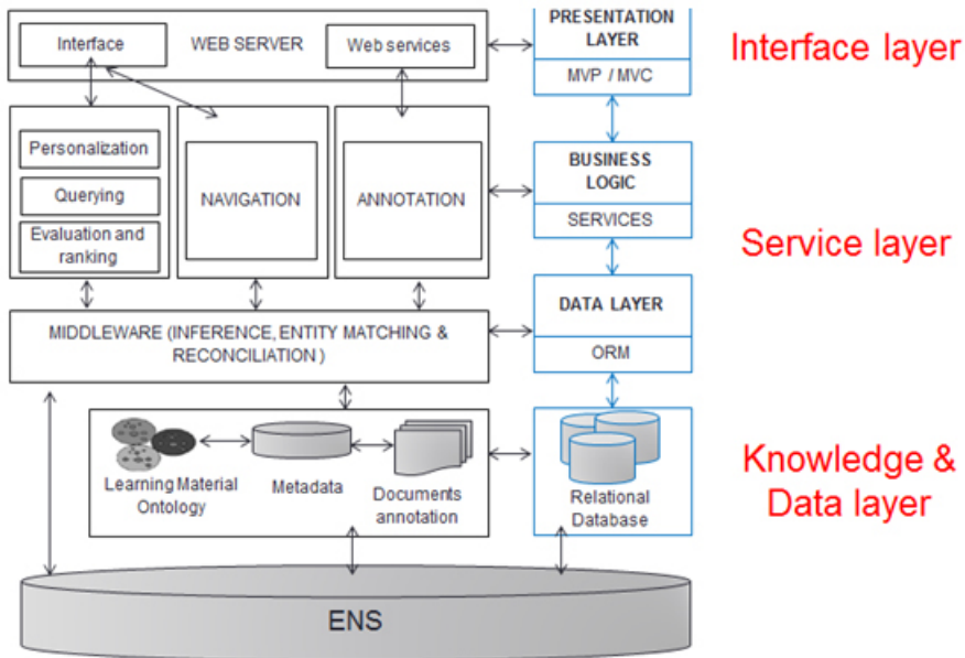
Fig. 4 - The OC semantically-enabled architecture
