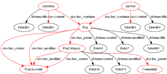
Fig.2 A partial view of SIOC ontology and the extensions added
