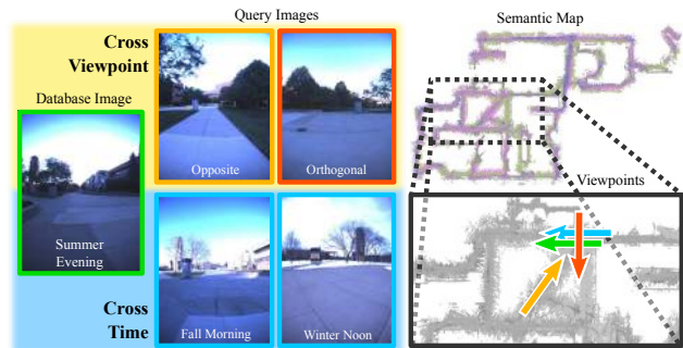
Figure 1: We propose a semantic localization technique which is able to match features over extreme appearance changes across viewpoints and time. In this example, the database contains only images captured in summer and from one particular viewpoint, yet our method correctly localizes images with strong viewpoint, illumination, and seasonal changes.
