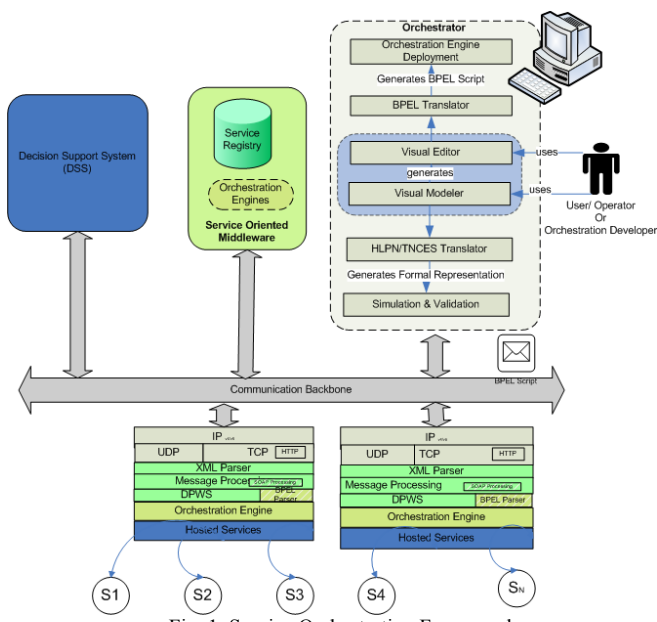
Fig. 1. Service Orchestration Framework
