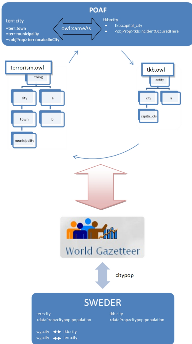
Figure 5: An example scenario
