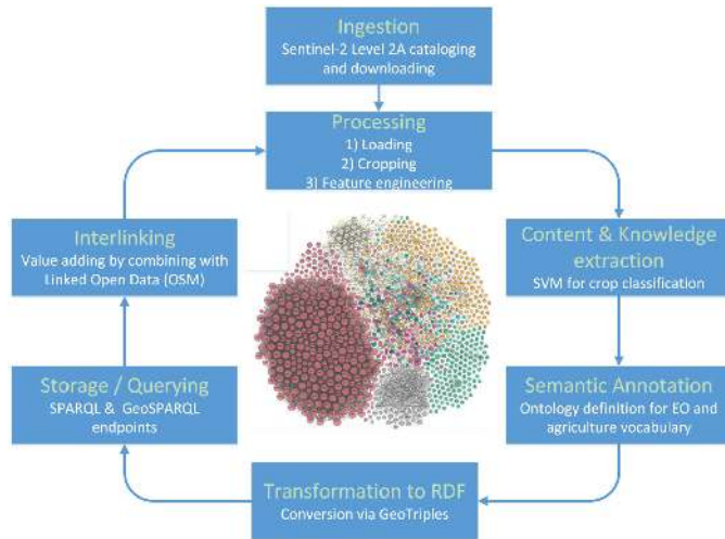
Fig. 1. Main stages of the complete life cycle of linked open EO data for the monitoring of the CAP.
