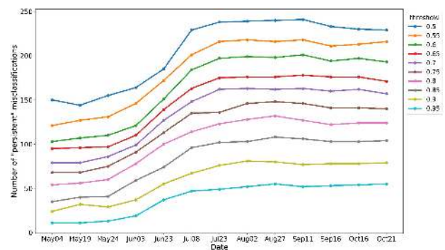
Fig. 8. Evolution of the number of constant persistent misclassifications for a varying threshold of the green category.
