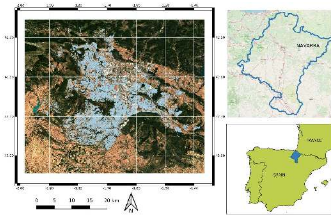
Fig. 3. Study area located in northeastern Spain and specifically in the Navarra district. The parcels of interest are shown in light blue color.
