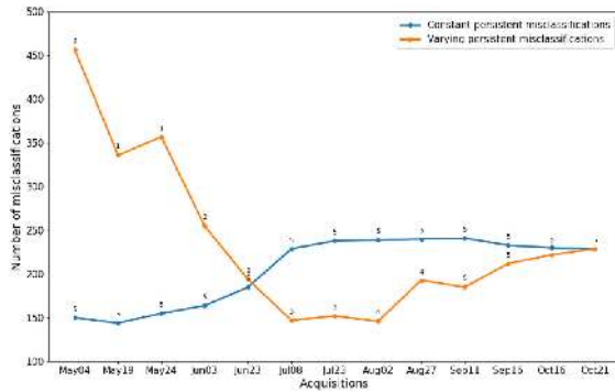
Fig. 9. Evolution of the number of misclassifications under constant (blue line) and varying thresholds (orange line). The varying threshold increases by one every two image acquisitions. The thresholds define which parcels are the misclassifications for each classification instance looking at the number of times they were found misclassified in previous runs.
