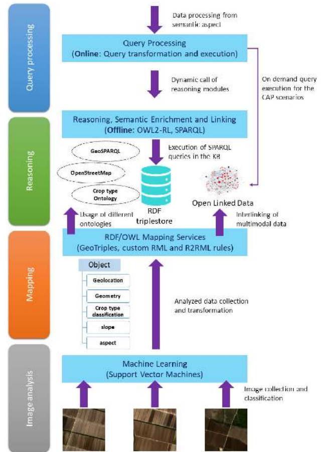
Fig. 2. System architecture overview.
