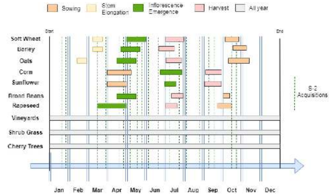
Fig. 4. Timeline of the growth cycle of major crops in Navarra, reworked from [8], together with the acquisition dates of the Sentinel-2 images.
