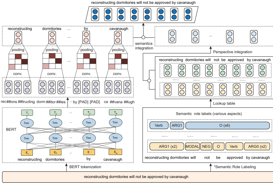
For the text, \{reconstructing\ dormitories\ will\ not\ be\ approved\ by\ cavanaugh\} , it will be tokenized to a subword-level sequence, \{rec, \#ons, \#ructing, dorm, \#itor, \#ies, will, not, be, approved, by, ca, \#vana, \#ugh\} . Meanwhile, there are two kinds of word-level semantic structures, [ARG1: reconstructing\ dormitories] [ARGM-MOD: will] [ARGM-NEG: not] be [V: approved] [ARG0: by\ cavanaugh] [V: reconstructing] [ARG1: dormitories] will\ not\ be\ approved\ by\ cavanaugh
