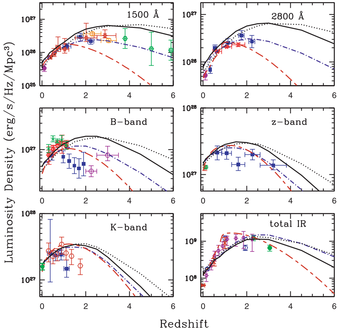
Figure 3. The luminosity density (integrated luminosity function of sources within a given redshift range) in our models versus redshift at 1500, 2800 Å, and in the B , z and K bands (approximately 4500, 9130 Å and 2.2 \mu\text{m} , respectively). The final panel on the lower right shows the total amount of energy that is absorbed and reradiated by dust at IR energies; units on the y-axis for this panel are solar luminosities per \text{Mpc}^3 . The solid black line is our WMAP5 prediction with evolving dust, and the dotted line are prior results from our \Lambda\text{CDM} model. Dash-dotted violet shows the predictions from our WMAP5 model using fixed dust attenuation parameters. The long-short dashed red line is the prediction of D11. Observational data shown here are as follows. 1500 Å: blue squares are from Dahlen et al. (2007), red stars are from Schiminovich et al. (2005), green stars are from Bouwens et al. (2007) and orange circles are from Reddy et al. (2008). The solid purple circle is a local measurement with GALEX by Wyder et al. (2005). 2800 Å: blue squares and the purple circle are again from Dahlen et al. (2007) and Wyder et al. (2005), respectively. Red stars are from Gabasch et al. (2006). B band: blue squares are from Dahlen et al. (2005). DEEP and COMBO-17 data from Faber et al. (2007) are shown as red stars and open red squares, respectively (these are very similar). This Combo-17 data is an update to that originally presented in Wolf et al. (2003), and we show the original points as green stars. The work of Marchesini et al. (2007) is shown as open purple hexes. z band: local measurements are provided by Montero-Dorta & Prada (2009) (red) and Blanton et al. (2003) (green). Blue squares are from Gabasch et al. (2006). K band: the local determination is from Kochanek et al. (2001). High-redshift data are from Barro et al. (2009) (blue squares) and Arnouts et al. (2007) (open red circles). Total IR luminosity: observational estimates of the IR emissivity are from Caputi et al. (2007) (open blue pentagons), Reddy et al. (2008) (green circles), Rodighiero et al. (2010) (purple stars) and Le Flocc'h et al. (2005) (red crosses).
