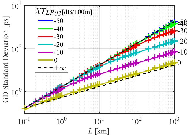
Fig. 7. Standard deviation of the GDs of the PMs as a function of transmission distance showing simulation results (markers) and analytical results (solid lines).
