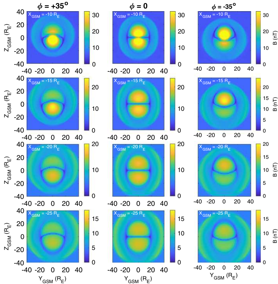
Fig. 12. Cross sections of the tail from the BATSUS model runs showing the magnetic field intensity, B . The rows are for X_{\text{GSM}} (=X_{\text{GSE}}) of (from top to bottom) -10 R_E , -15 R_E , -20 R_E , and -25 R_E . The columns are for dipole tilts \phi of (left) +35^\circ , (middle) 0 and (right) -35^\circ . The outer ring is the bow shock and the two tail lobes, separated by the low-field plasma sheet can be clearly seen. At all X_{\text{GSM}} , the field in the “winter” lobe (south for \phi = +35^\circ , north for \phi = -35^\circ ) is similar to that for the \phi = 0 case (and sometimes very slightly enhanced), whereas for the “summer” lobe (north for \phi = +35^\circ , south for \phi = -35^\circ ) it is always considerably lower.
