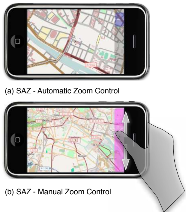
Figure 2: Placement and visualization of the zoom level slider in the SAZ map interface: (a) shows the SAZ interface in automatic zooming mode (no touch on slider), (b) shows the manual zooming mode (finger on slider thumb controls the zoom level).
