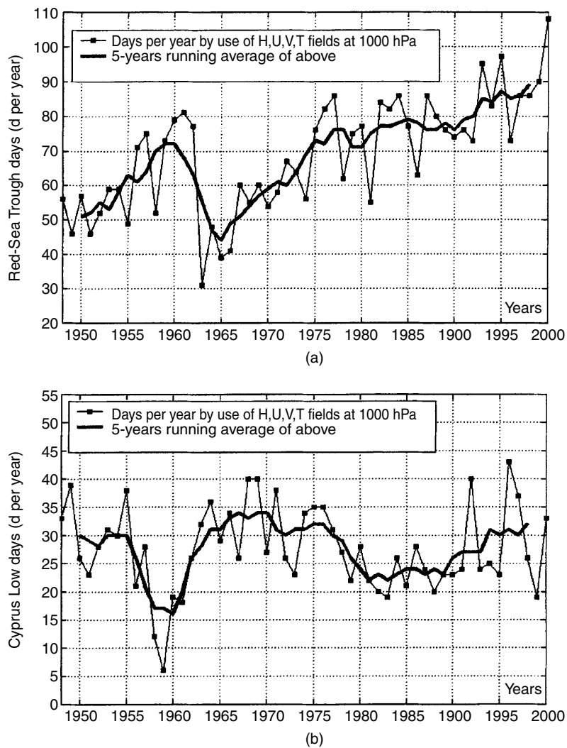
Figure 2. Annual numbers of days (frequencies) for 1948–2000: (a) RST; (b) Cyprus low. Thin lines with squares indicate results obtained by use of H , T , U , V fields at 1000 hPa level. Heavy lines are the 5 year running averages
