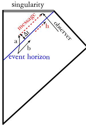
Fig. 2. The duplication experiment. a and b are a pair of correlated spins. The observer sees h , which is a copy of a after the information retention time via Hawking radiation. To see a , a should be sent to the out-going direction after the time \Delta t . If the observer sees both a and h , since they are both correlated to b , it violates the no-cloning theorem and unitarity.
