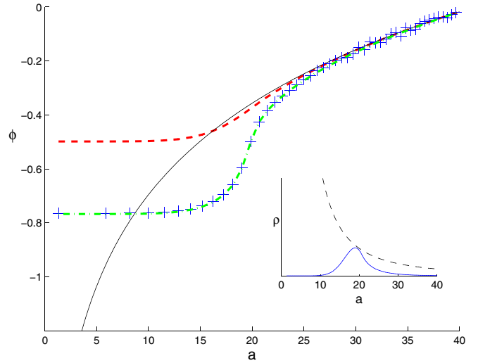
FIG. 4 (color online). Evolution for J = 500 , P_\phi = 1600l_p . The classical (solid line) and ET-I trajectory (dashed line) deviate from quantum evolution (+ line) for scale factors at which perturbative corrections become significant. ET-II agrees with evolution from the quantum constraint until a_0 . Inset: ET-II corrections become significant when the matter density (solid line) approaches the critical density (dashed line).
