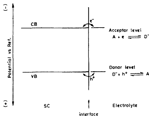
Figure 4. Location of energy levels for charge-transfer in the absence of surface states. For efficient charge-transfer the donor and acceptor levels should lie within \pm kT ( = 0.026 eV at 300 K) from the valence and conduction band edge energies (after Gerischer 1970).
