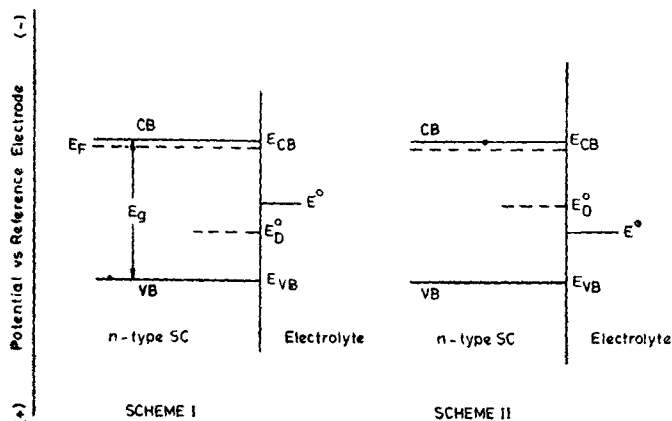
Figure 9. Interface energetics for n -type SC/electrolyte junction, taking into account of the decomposition potential, E_D^0 , of the sc. Scheme I: Situation for E_{redox} (= E^0) more negative than E_D^0 . In this case, the primary oxidation product, 'OX' (from the reaction Red + h^+ \rightarrow OX ) is not capable (thermodynamically) of oxidizing the sc. If 'Red' can successfully capture 100% of the photogenerated holes, sc will be completely stable to photoanodic dissolution. Scheme II. E_{redox} is more positive than E_D^0 . Oxidized form of the redox couple, 'OX' (with a redox potential E_{redox} ), is capable (thermodynamically) of spontaneously oxidizing the sc in dark.
