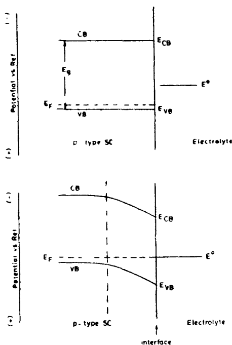
Figure 3. p -type SC/electrolyte interface energetics: a. SC before contacting the electrolyte. b. SC in charge-transfer equilibrium with the electrolyte.
