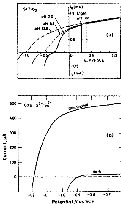
Figure 10. Typical current-voltage ( i-v ) characteristics of (a) n -SrTiO 3 single crystal electrode under (anodic polarization) illumination ( h\nu \geq 3.2 eV). Dependence of photocurrent onset potential with pH is also shown (after Watanabe et al 1976); (b) n -CdS single crystal electrode in 1 M Na 2 S-1 M S-1 M NaOH (after Ellis et al 1976). The potential of photocurrent onset, E_{onset} , can be taken as the flat-band potential, E_{fb} , at sufficiently high light intensities. The saturation of photocurrent (potential independent behaviour) is due to the light intensity limited minority carrier generation. Efficient electron-hole pair separation in the space charge layer and charge transfer across the interface are characterized by a steep rise in photocurrent and a high saturation value.
