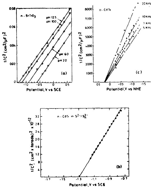
Figure 6. Plots of (differential capacitance) -2 vs applied potential (at the sc electrode) (Mott-Schottky plots) for calculation of E_{fb} and N_d (carrier concn.). a. n\text{-SrTiO}_3 (aq. electrolytes at different pH values) (after Watanabe et al 1976). b. n\text{-CdS} in polysulfide electrolyte (after Ellis et al 1977). c. p\text{-CdTe} in 1 M NaOH (at various impressed a z frequencies) (after Ohashi et al 1977b).
