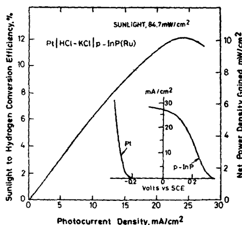
Figure 12. The high efficiency photoassisted water electrolysis cell, Pt/1 M HCl-2M KCl/ p -InP(Ru). This cell represents the most efficient (12%) system for the direct conversion of sunlight into the storable fuel, H 2 . This cell works under an applied bias. However, the long term stability is yet to be established. Solar-to-hydrogen conversion efficiency and power density gain as a function of photocurrent density are shown. The current-voltage characteristics of a platinum and a p -InP (Ru) photocathode at the above sunlight intensity are compared in the inset. With p -InP (Ru) photocathode, H 2 -evolution starts at +0.36 V vs the SCE or 0.64 V vs oxygen electrode. Platinum requires -0.23 V vs SCE or 1.23 V vs oxygen (after Heller and Vadimsky 1981).
