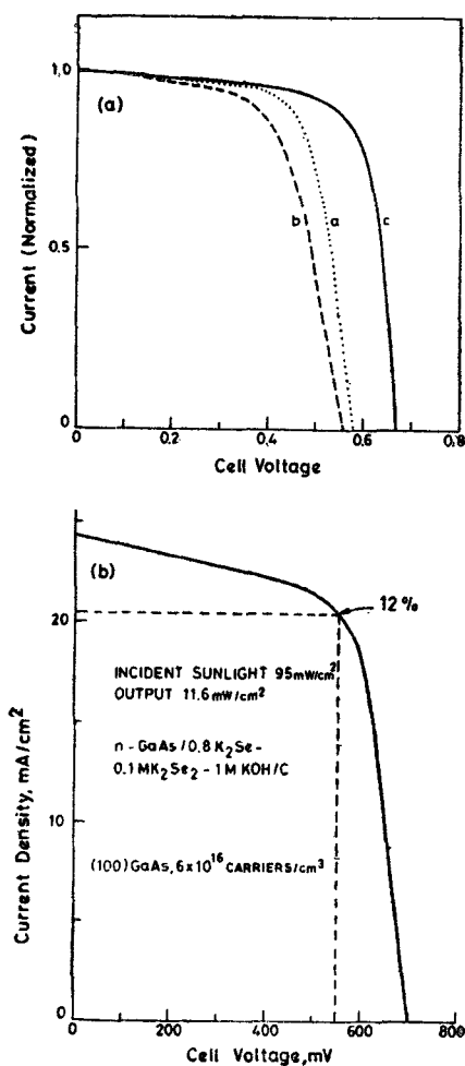
Figure 13. High efficiency (12%) sc/liquid junction (regenerative) solar cell with a photoanode, n -GaAs/0.8 M K 2 Se-0.1 M K 2 Se 2 -1 M KOH/C (graphite). (a) Power characteristics of the cell and the changes effected by surface treatment (modification) of n -GaAs with Bi 3+ and Ru 3+ ions are shown. Curve (a): Freshly etched electrode (etchant: 1:1 of 30% H 2 O 2 -conc. H 2 SO 4 ) followed by dip in the redox couple soln. (I). Curve (b): I followed by dip in bismuth solution (0.01 M Bi 3+ + 0.1 M HNO 3 ). Curve (c): I followed by dip in ruthenium soln. (0.01 M Ru 3+ + 0.1 M HNO 3 ). (b) Same as curve (c) of figure 13a with the actual data. As can be seen, Ru 3+ has beneficial effect. Various other metal ions also have been examined but Ru 3+ shows the best effect (after Parkinson et al 1978a, b).
