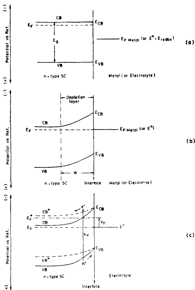
Figure 2. SC/electrolyte interface energetics; a. n -type SC before contacting a metal or electrolyte (flat-band situation, E_F = E_{t_b} ). b. n -type SC in charge-transfer equilibrium with a metal (or electrolyte). c. n -type SC/electrolyte interface under illumination with h\nu \geq E_g . Asterisk indicates the steady state situation under illumination. Light generated holes move towards the surface whereas the electrons move towards the bulk of SC [ E_{CB} , E_{VB} , the energies corresponding to the bottom of the conduction band and top of the valence band; E_F and E_{F, \text{metal}} Fermi levels of the SC and metal; E^0 or E_{\text{redox}} , the standard electrochemical potential (= Fermi level) of the electrolyte; E_g , the band gap of the SC; W , the width of the depletion layer; V_p , the photopotential].
