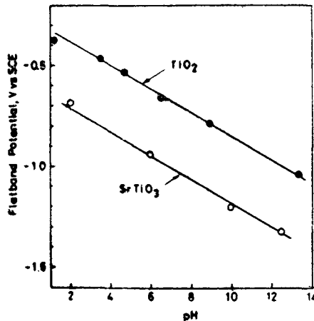
Figure 5. Variation of E_{fb} with pH of the electrolyte for n\text{-SrTiO}_3 and n\text{-TiO}_2 electrodes. From the slope, it follows that E_{fb} varies by 0.059 V/unit pH (after Watanabe et al 1976).
