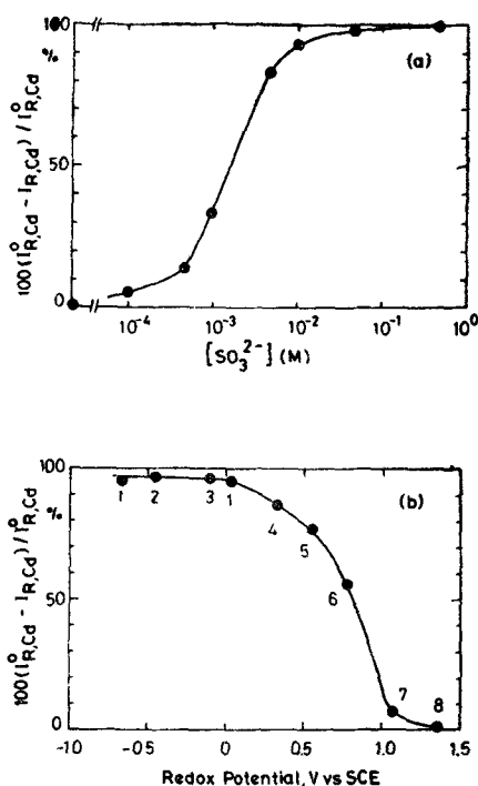
Figure 11. Percentage dissolution (photocorrosion) suppression of CdS electrode determined by rotating ring disc electrode techniques (disc : CdS single crystal ; ring : amalgamated Cu ring). (a) Percentage of dissolution suppression as a function of aq \text{SO}_3^{2-} concentration (dissolution reaction: \text{CdS} + 2h^+ \rightarrow \text{Cd}^{2+} + \text{S} ). (b) Percentage of dissolution suppression by reducing agents (conc. for all 0.01 M) as a function of their redox potential
