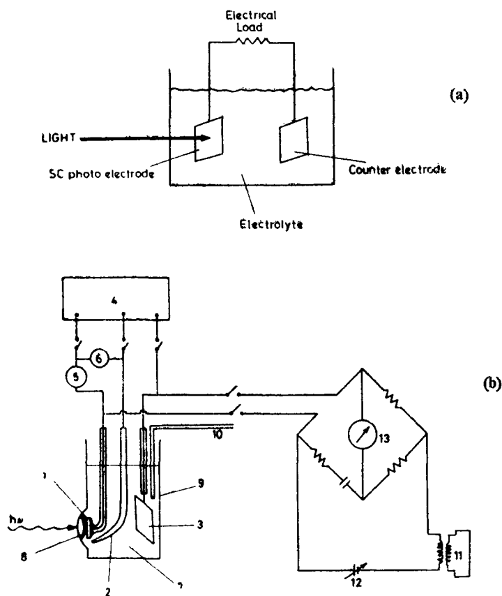
Figure 1. a. Schematic representation of a photoelectrochemical cell (PEC). b. Standard 3-electrode set-up for current-voltage ( i - v ) and capacitance ( C ) measurements. 1. Semiconductor (sc) electrode. 2. Saturated calomel 1 electrode (SCE). 3. Platinum (counter) electrode. 4. Potentiostat. 5. Ammeter. 6. D.C. voltmeter. 7. Electrolyte. 8. Optical window for illumination of the sc photoelectrode. 9. Glass cell. 10. Gas bubbler. 11. Oscillator. 12. power supply. 13. Null detector.
