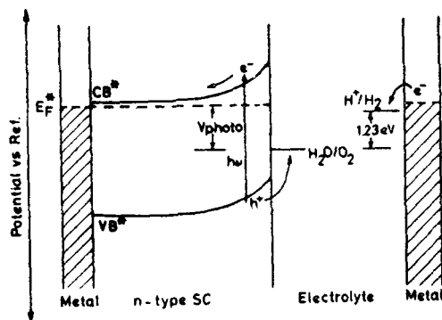
Figure 7. Energetics for a water photoelectrolysis cell employing an n -type sc. Asterisk indicates steady state situation under illumination. V_{\text{photo}} is the open-circuit photopotential of the cell. At anode: \text{H}_2\text{O} + h\nu \rightarrow \frac{1}{2}\text{O}_2 + \text{H}^+ ; at cathode: \text{H}^+ + e^- \rightarrow \frac{1}{2}\text{H}_2 .
