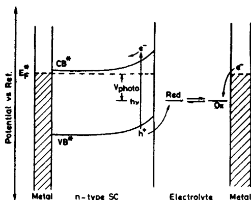
Figure 8. Energetics for an n -type SC/electrolyte junction (regenerative) solar cell. Asterisk indicates the steady state situation under illumination. V_{\text{photo}} is the open-circuit photopotential of the cell. At anode: \text{Red} + h^+ \rightarrow \text{OX} ; at cathode: \text{OX} + e^- \rightarrow \text{Red} .
