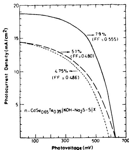
Figure 15. Photocurrent-voltage (power) characteristics of the sc/liquid junction solar cell: n-CdSe_{0.65}Te_{0.35}/KOH-Na_2S-S (all 1 M)/X. (X = sulfide impregnated brass gauze). Area of the photoanode, 0.22 \text{ cm}^2 . Simulated sunlight (0.85 of AM1 radiation). Efficiency and fill factor values are shown. The curves show the effect of etch treatment: dashed curve, HCl: HNO_3 etch; broken curve, CrO_3 etch and K_2CrO_4 treatment; full curve, photoetch in the electrolyte followed by treatment with K_2CrO_4 solution (after Hodes 1980).
