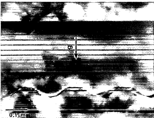
FIG. 2. A TEM photograph of the cross-sectional view of a 6-QW \text{In}_{0.6}\text{Ga}_{0.4}\text{As} (5 nm)/ Q_{1.25} (18.6 nm) active-layer DFB laser with a 2-QW \text{In}_{0.62}\text{Ga}_{0.38}\text{As} (4 nm)/InP (9.3 nm) grating.
