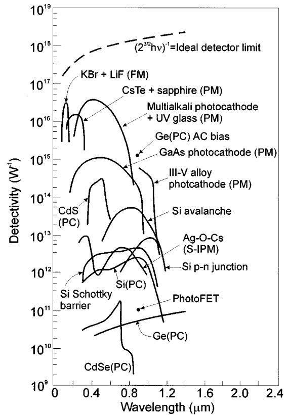
FIG. 14. Detectivity vs wavelength values of 0.1–1.2 \mu\text{m} photodetectors. PC indicates a photoconductive detector and PM indicates a photomultiplier. Detector areas are given in Table II (after Ref. 26).
