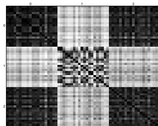
Figure 3: Normalized Gram matrix computed with the linear IGV kernel of twenty images of “0”, “1” and “2” displayed in that order. Darker spots mean values closer to 1, showing that the restriction to “0” and “1” yields good separation results, while “0” and “2” can hardly be discriminated using variance analysis.
