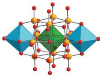
Fig. 9 Structure of the mixed-valent [V_2^{IV}V_{12}^{VO}O_{40}(GeOH)_8]^{8-} polyoxoanion, as present in K_2Na_6[V_{14}GeO_{40}] \cdot 10H_2O . Colour code: O, red; Ge, green; V^{IV/O_x} , sky-blue polyhedra; V^V , light orange.
