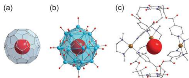
Fig. 5 The \text{H}_2\text{O} -endothedral complexes of \text{C}_{60} (a), 63 the “fully-reduced” [\text{V}_{18}\text{O}_{42}]^{12-} POV (b), 45,64 and [\text{Pd}_3\text{L}_2]^{6+} (c). 61 C, grey; N, blue; O, red; \text{V}^{\text{IV}} , sky blue; Pd, brown.
