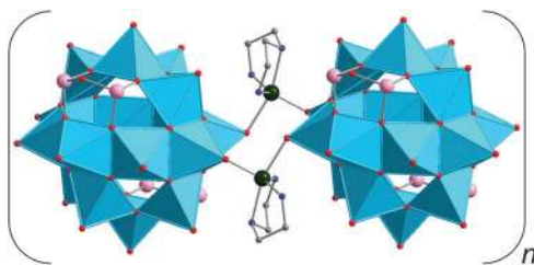
Fig. 20 Polyhedral representation of a segment of the polymeric structure of [\text{Zn}_2(\text{dien})_3]_n[(\text{Zn}(\text{dien})_2\text{V}_{16}\text{As}_4\text{O}_{42}(\text{H}_2\text{O}))]:3\text{H}_2\text{O} . Colour code: C, grey; N, blue; As, rose; O, red; \text{V}^{\text{IV}}\text{O}_x , sky-blue polyhedra; Zn, dark green.
