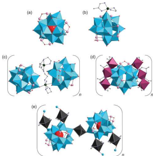
Fig. 19 (a) The “fully-reduced” [\text{H}_2\text{O}@V_{15}\text{As}_6\text{O}_{42}]^{6-} polyoxoanion. (b) The “fully-reduced” \{[\text{Zn}(\text{en})(\text{enMe})\}\text{V}_{15}\text{As}_6\text{O}_{42}\}^{4-} hybrid polyoxoanion. Hydrogen atoms and encapsulated water molecule are not shown. (c) A segment of the polymeric structure of [\text{Zn}_2(\text{dien})_3(\text{H}_2\text{O})_2]_{0.5}[\text{V}_{15}\text{As}_6\text{O}_{42}(\text{H}_2\text{O})] \cdot 2\text{H}_2\text{O} . (d) A segment of the extended solid-state structure of [\text{Co}(\text{enMe})_2]_3[\text{V}_{15}\text{As}_6\text{O}_{42}(\text{H}_2\text{O})] \cdot 2\text{H}_2\text{O} . (e) A segment of the extended solid-state structure of [\text{Cu}(\text{en})_2]_{1.5}[\text{H}_3\text{V}_{15}\text{As}_6\text{O}_{42}(\text{H}_2\text{O})] \cdot 3\text{H}_2\text{O} . Colour code: C, grey; N, blue; As, rose; O, red; V^V , sky blue; V^V\text{O}_x , sky-blue polyhedra; Co, plum; Cu, black; Zn, dark green.
