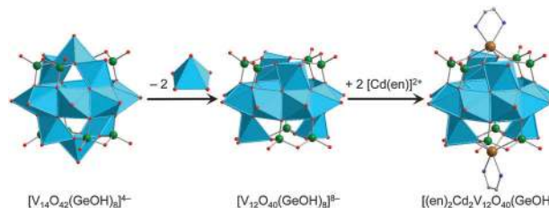
Fig. 10 Schematic design of the TMC-supported, “fully-reduced” hybrid polyoxoanion [Cd_2(en)_2V_{12}O_{40}(GeOH)_8]^{4-} (right). This tetraanion is formed when two \{VO\}^{2+} caps situated between the \{Ge_2O_7\} groups in \alpha - [V_{14}O_{42}(GeOH)_8]^{4-} (left) are replaced with two [Cd(en)]^{2+} fragments. Encapsulated water molecule and hydrogen atoms are not shown. Colour code: Ge, green; N, blue; O, red; V^{IV/O_x} , sky-blue polyhedra; Cd, brown.
