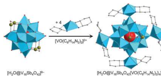
Fig. 26 The “fully-reduced” [H_2O@V_{16}Sb_4O_{42}(VO(dach)_2)_4] self-assembly (right) and its constituents, [H_2O@V_{16}Sb_4O_{42}]^{6-} (left) and [VO(dach)_2]^{2+} (middle). Hydrogen atoms are not shown. Colour code: C, grey; N, blue; Sb, dark yellow; O, red; V^{IV}O_x , sky-blue polyhedra.
