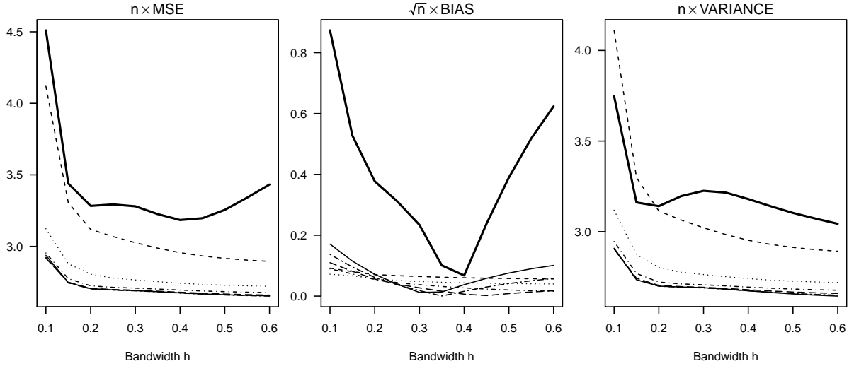
Figure 1: Simulation results: MSE, absolute bias and variance of the IPW estimator for various values of h (bold solid line), compared to results for the DR estimator with bandwidth g equal to .035 (short-dashed line), .065 (dotted line), .095 (dot-dashed line), .125 (long dashed line), .155 (long dashed dotted line), and .185 (thin solid line).
