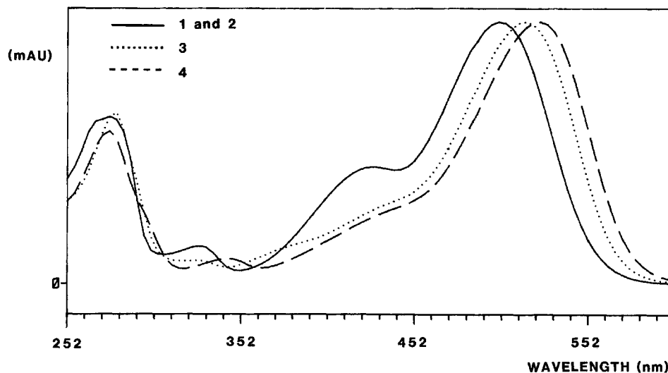
Fig. 1. Spectra of anthocyanins found in receptacles and seeds of D. dactyloides recorded with a diode-array detector during HPLC analysis. Automatic scaling was used.
