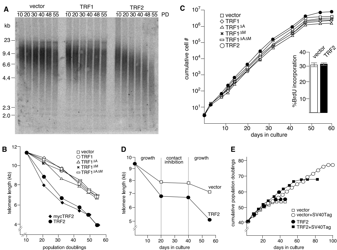
Fig. 1. Effect of TRF2 overexpression on telomere shortening and culture growth.
