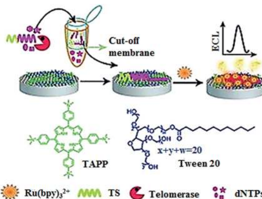
Fig. 5 Label-free electrochemiluminescent detection of telomerase activity using porphyrin-functionalized graphene. Adapted with permission from ref. 41, Copyright 2012 WILEY-VCH Verlag GmbH & Co. KGaA, Weinheim.
