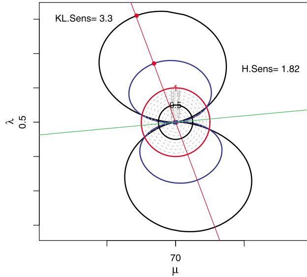
Figure 2: Comparison of local sensitivity methods in the plane spanned by parameters \mu and \lambda centered at \gamma_0 = (\mu_0, \lambda_0) = (70, 0.5) . Red and green lines: eigenvectors provided by the infinitesimal local approach based on the Kullback-Leibler divergence with the principal eigenvalue (worst-case sensitivity) 3.284. Black curve: circular sensitivity in each direction provided by the \epsilon -local approach for \epsilon_0 = 5e-05 based on the Kullback-Leibler divergence. Blue curve: circular \epsilon -local sensitivity based on the Hellinger distance for \epsilon_0 = 0.00354 . In both cases the choice of \epsilon_0 corresponds to a shift in means by 0.01 with respect to the unit-variance normal distribution. The worst-case sensitivities provided by the \epsilon -local approaches are indicated by a red dot. The scale for sensitivity values (0.1, 0.2, ..., 0.9, 1) is indicated by grey circles. Sensitivity equal to 0.5 is marked by a black circle, whereas the value 1 is marked by a red one.
