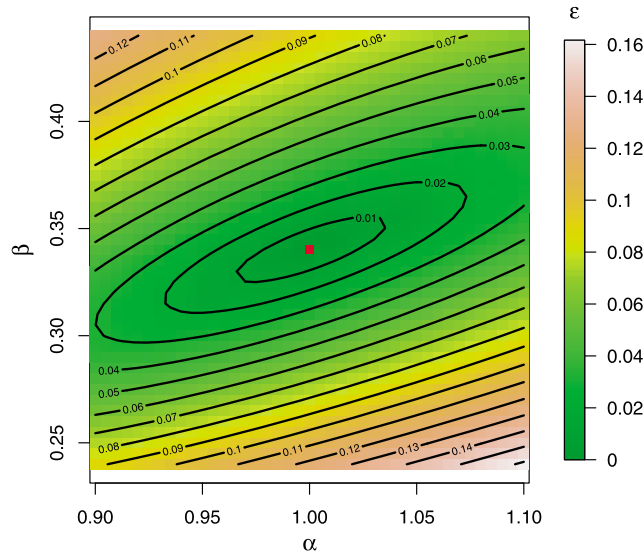
Figure 1: Contour plots of G_{\gamma_0}(\epsilon) for gamma distribution with center \gamma_0 = (\alpha_0, \beta_0) = (1, 0.34) based on the Hellinger distance.
