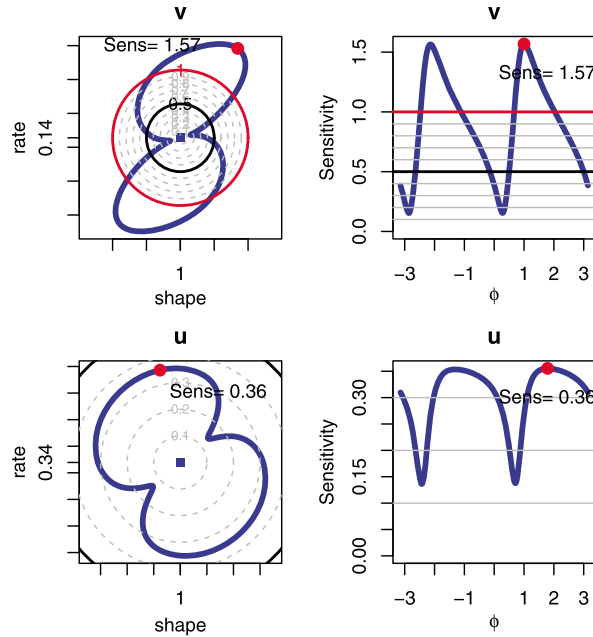
Figure 4: Polar sensitivity plots (left) centered at \gamma_0 and sensitivity plots rolled out on the line (right) in each polar direction of the circular S_{\gamma_0}^c(\epsilon_0) together with the worst-case sensitivity S_{\gamma_0}(\epsilon_0) (red dot) for \tau_v at \gamma_0^{(v)} (top) and \tau_u at \gamma_0^{(u)} (bottom) components in model (13) in Section 5 for \epsilon_0 = 0.00354 . The scale for sensitivity values (0.1, 0.2, ..., 0.9, 1) is indicated by grey circles and lines, respectively. Sensitivity equal to 0.5 is marked by a black colour, whereas the sensitivity value 1 is marked by a red one.
