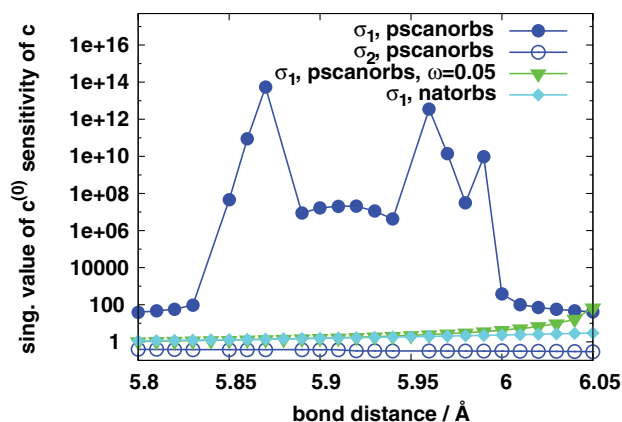
FIG. 3. Singular values of the coefficient sensitivity matrix Eq. (45) around 6 Å internuclear distance, for the ground state of the LiH molecule in MP partitioning. The largest singular value is denoted by \sigma_1 , the second largest is \sigma_2 . Basis set and reference function agrees with that of Fig. 1. The nature of orbitals (pscanorb: pseudo-canonicals; natorbs: naturals) is varied. Symbol \omega refers to Tikhonov damping (c.f. Eq. (17)) and gives the value of the damping parameter.
