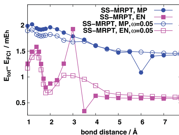
FIG. 1. Errors of second order SS-MRPT energies for the ground state of the LiH molecule in Dunning's DZP basis (Ref. 24). Reference function is CAS(2,5), active orbitals are pseudo-canonicals. Full CI values are subtracted from total SS-MRPT energies. Partitioning is either MP or EN. Filled symbols correspond to undamped equations, results obtained by Tikhonov damping according to Eq. (17) are shown by hollow symbols. The damping parameter is denoted by \omega .
