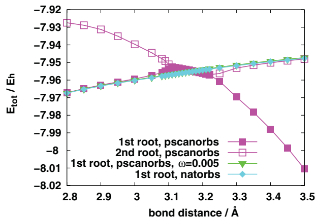
FIG. 5. Same as Fig. 2 in EN partitioning, around 3 Å bond distance.
