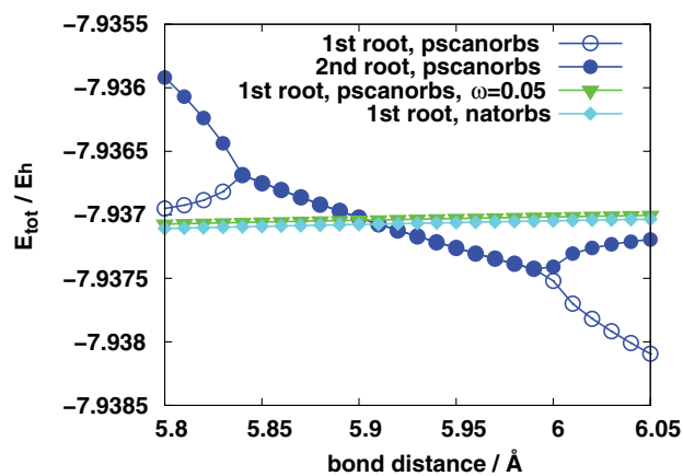
FIG. 2. Total energy of the ground state of the LiH molecule as a function of the internuclear distance, obtained by second order SS-MRPT in MP partitioning. Basis set and reference function agrees with that of Fig. 1. The nature of orbitals (pscanorb: pseudo-canonicals; natorbs: naturals) is varied. Whenever Tikhonov damping is used [cf. Eq. (17)] symbol \omega is indicated and shows the value of the damping parameter. Both roots of the second-order Hamiltonian \mathbf{H}^{[2]} are shown for the undamped equations, displayed by circles.
