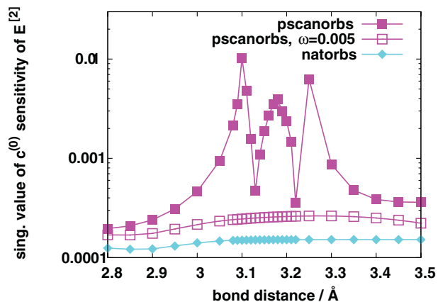
FIG. 7. Same as Fig. 4 in EN partitioning, around 3 Å bond distance.
