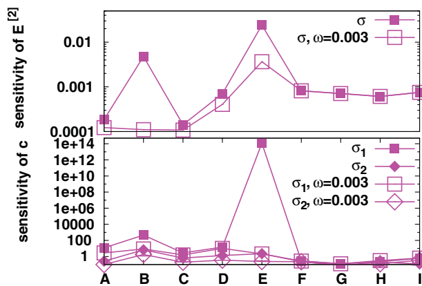
FIG. 10. Same as Fig. 9 in EN partitioning.
