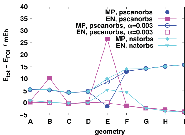
FIG. 8. Errors of second order SS-MRPT energies for the ground state of the BeH 2 system in DZ basis (see text for more detail). Reference function is CAS(4,4), active orbitals are either pseudo-canonical (pscanorb) or natural (natorbs). Full CI values are subtracted from total SS-MRPT energies. Partitioning is either MP or EN. Filled symbols correspond to undamped equations, results obtained by Tikhonov damping according to Eq. (17) are shown by hollow symbols. The damping parameter is denoted by \omega .
