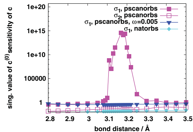
FIG. 6. Same as Fig. 3 in EN partitioning, around 3 Å bond distance.
