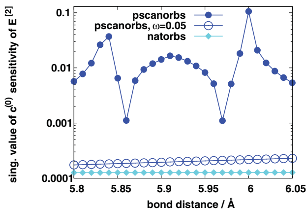
FIG. 4. Nonzero singular value (i.e. norm) of the coefficient sensitivity matrix Eq. (43), around 6 Å internuclear distance, for the ground state of the LiH molecule in MP partitioning. Basis set and reference function agrees with that of Fig. 1. The nature of orbitals (pscanorb: pseudo-canonicals; natorbs: naturals) is varied. Symbol \omega refers to Tikhonov damping (c.f. Eq. (17)), and gives the value of the damping parameter.
