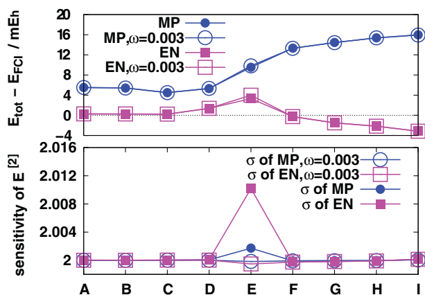
FIG. 11. Analysis of the unrelaxed second order SS-MRPT energy, E^{[2]} = \langle \Phi | H^{[2]} | \Phi \rangle for the ground state of the BeH 2 system in DZ basis. Reference function is CAS(4,4), active orbitals are pseudo-canonicals. Filled symbols correspond to undamped equations, results obtained by Tikhonov damping according to Eq. (17) are shown by hollow symbols. The damping parameter is denoted by \omega . Energy errors are shown in the upper plot. Nonzero singular value (i.e. norm) of the coefficient sensitivity of the unrelaxed E^{[2]} is shown in the bottom plot.
