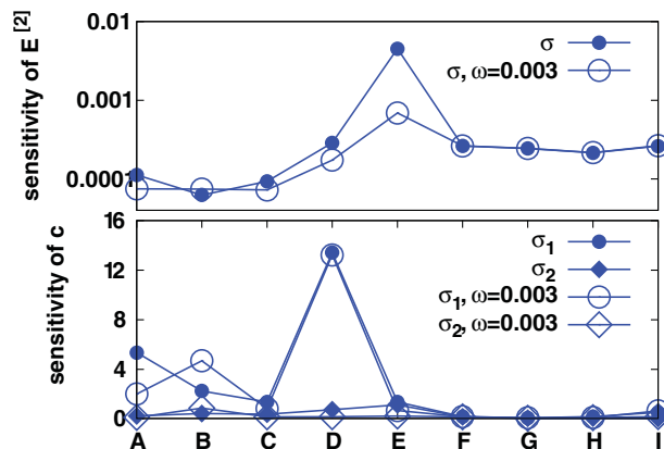
FIG. 9. Nonzero singular value (i.e. norm) of the coefficient sensitivity matrix Eq. (43) (upper plot) and the two largest singular values of the coefficient sensitivity matrix Eq. (45) (bottom plot) for the ground state of the BeH 2 system in MP partitioning, using pseudo-canonical active orbitals. Basis set and reference function agrees with that of Fig. 8. Symbol \omega refers to Tikhonov damping (c.f. Eq. (17)) and gives the value of the damping parameter.
