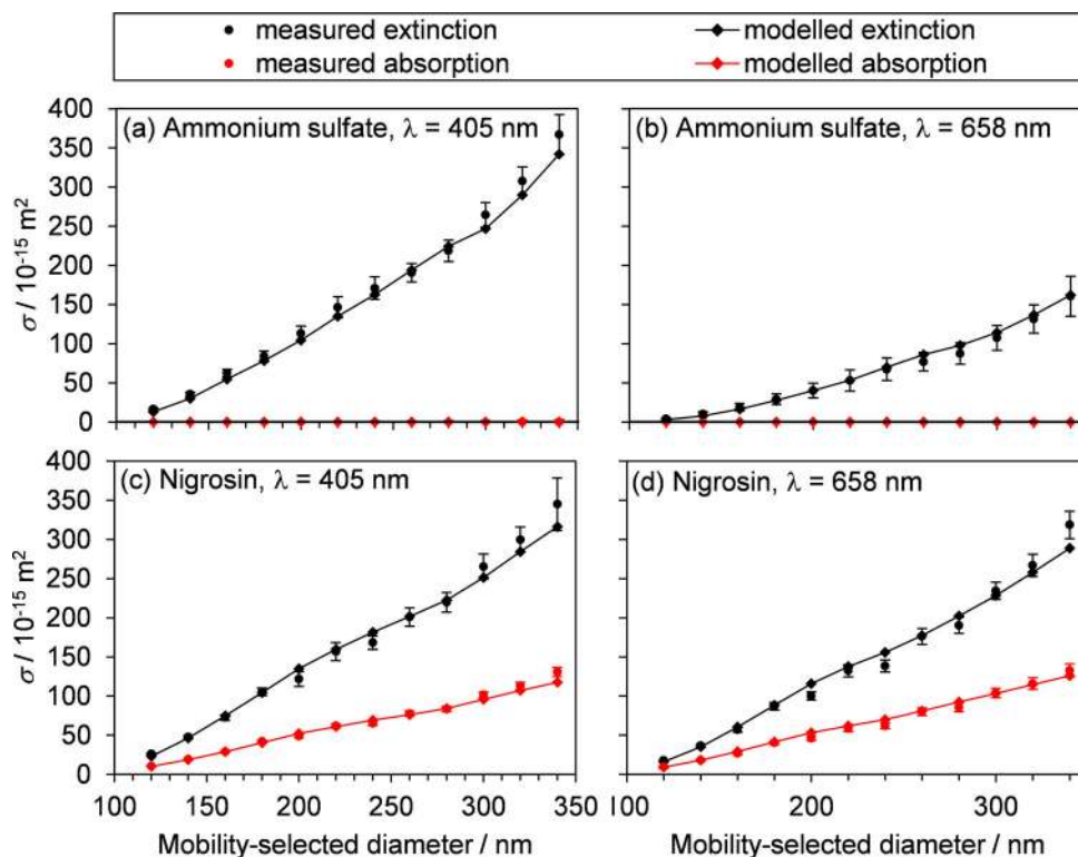
Figure 2. Comparison of measured \sigma_{\text{ext}} and \sigma_{\text{abs}} with model values using the literature RI for (a),(b) AS (Toon et al. 1976), and (c),(d) nigrosin (Bluvshstein et al. 2017). Measurements are shown for both spectroscopy wavelengths of 405 and 658 nm. Vertical error bars represent one standard deviation in the measured cross sections. Lines between model cross section values are to guide the eye only.
