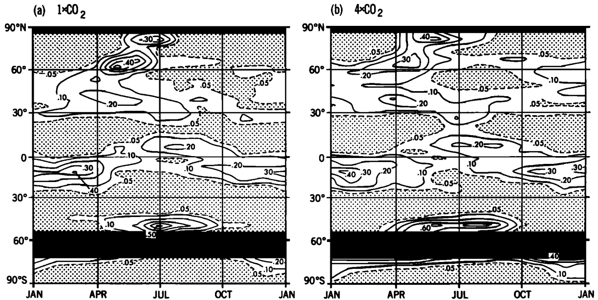
Fig. 29. Latitude-time distribution of zonal mean runoff rate over continents. (a) 1 \times \text{CO}_2 experiment, (b) 4 \times \text{CO}_2 experiment. Units are in centimeters per day.
