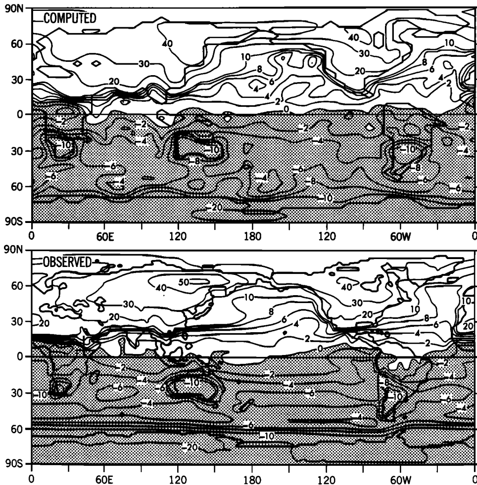
Fig. 8. Geographical distribution of surface air temperature difference (degrees Kelvin) between August and February. Top: computed distribution from the 1 \times \text{CO}_2 experiment. Bottom: observed distribution (from the data compiled by Crutcher and Meserve [1970] and Taljaad et al. [1969]). Note that the contour interval is 2^\circ\text{K} when the absolute value of the difference is less than 10^\circ\text{K} and is 10^\circ\text{K} when it is more than 10^\circ\text{K} .
