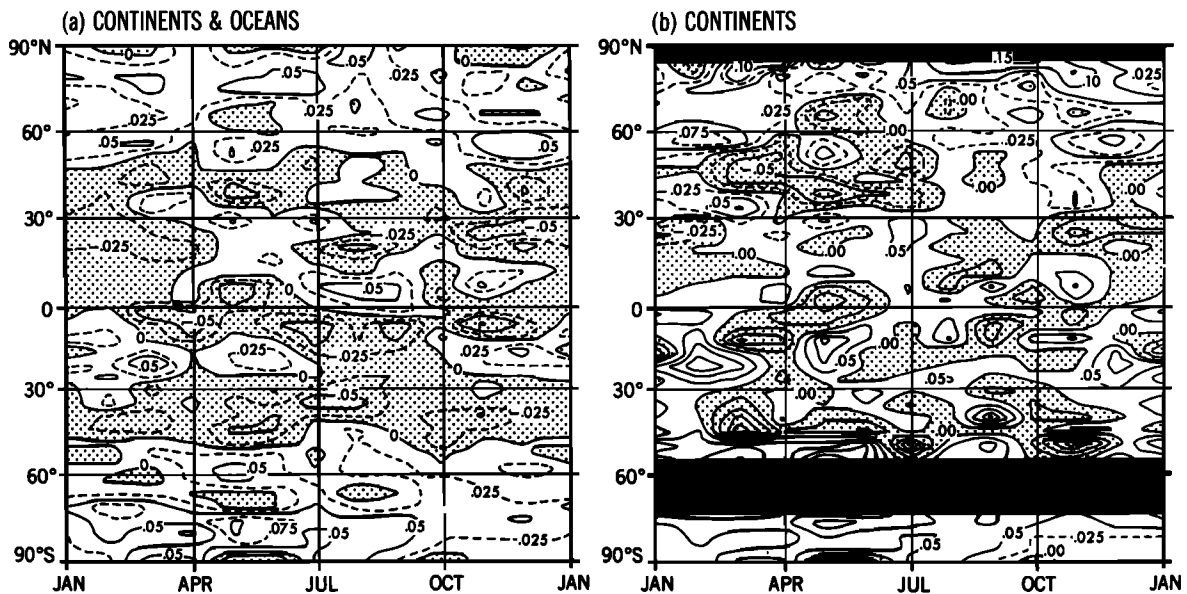
Fig. 26. Latitude-time distribution of zonal mean difference in (P - E) between the 4 \times \text{CO}_2 and 1 \times \text{CO}_2 experiments. (a) Continents and oceans and (b) continents. Units are in centimeters/day. The areas of negative (P - E) are shaded.
