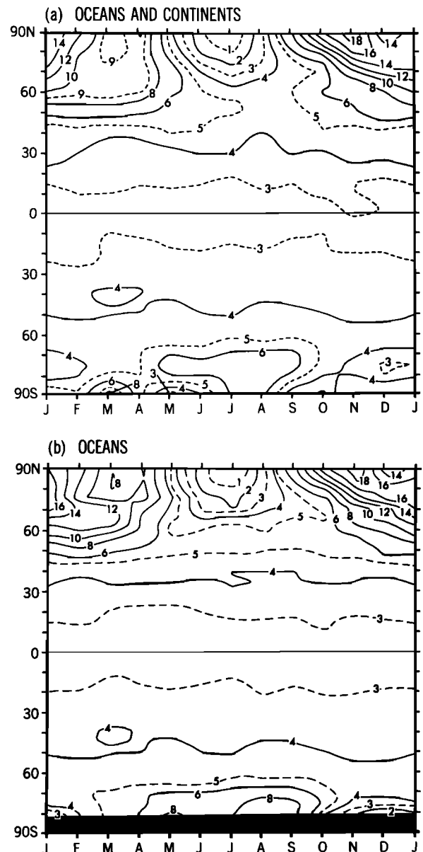
Fig. 16. Latitude-time distribution of zonal mean difference in surface air temperature (degrees Kelvin) between the 4 \times \text{CO}_2 and 1 \times \text{CO}_2 experiment. (a) Oceans and continents, (b) oceans, and (c) continents. The difference is computed at the lowest finite difference level located at about 70 m above the earth's surface.
