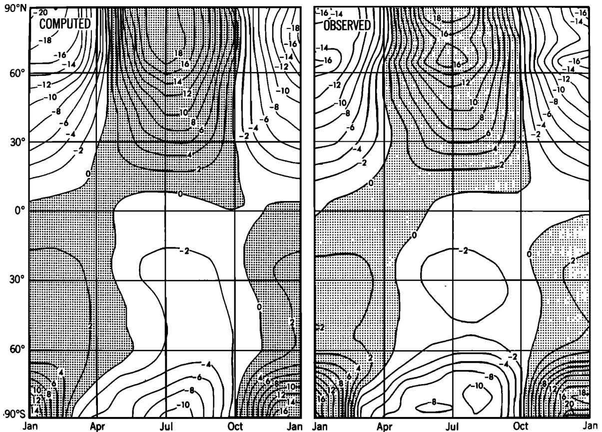
Fig. 9. Latitude-time distributions of deviations in the zonal mean surface air temperature from the annual mean value (degrees Kelvin). Left: computed distribution from the 1 \times \text{CO}_2 experiment. Right: observed distribution (obtained from the data compiled by Crutcher and Meserve [1970]; Taljaad et al. [1969]).
