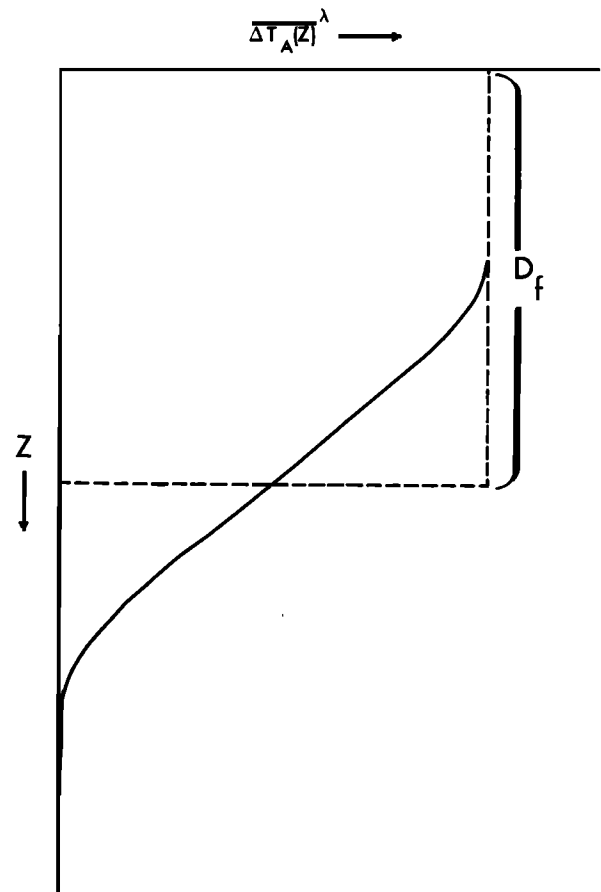
Fig. 2. Schematic diagram illustrating the method for determining the effective depth of the mixed layer ocean.
