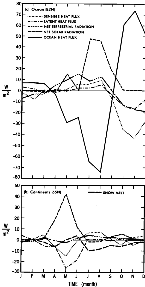
Fig. 19. Annual marches of the zonal mean differences in various heat balance components at the earth's surface between the 4 \times \text{CO}_2 and 1 \times \text{CO}_2 experiments. (a) Ocean surface at 82^\circ\text{N} , (b) continental surface at 65^\circ\text{N} . Positive difference indicate an additional flux towards the surface. Units are in \text{W m}^{-2} .
