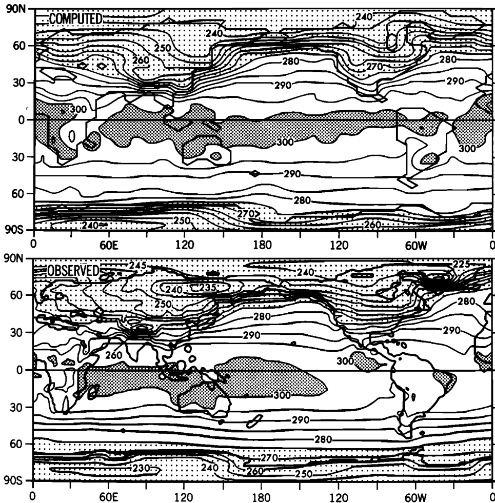
Fig. 7a. Geographical distributions of monthly mean surface air temperature (degrees Kelvin) in February. Top: computed distribution from the 1 \times \text{CO}_2 experiment. Bottom: observed distribution [Crutcher and Meserve, 1970; Taljaad et al. , 1969]. The computed surface air temperature represents the temperature of the model atmosphere at the lowest finite difference level located at about 70 m above the earth's surface.
