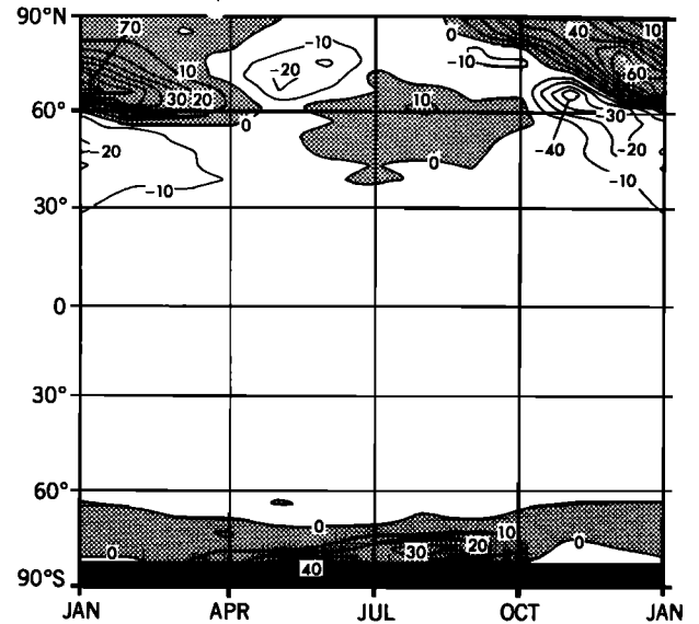
Fig. 20. Latitude-time distribution of zonal mean difference in the upward flux of sensible heat ( \text{W m}^{-2} ) over model oceans between the 4 \times \text{CO}_2 and 1 \times \text{CO}_2 experiment.
