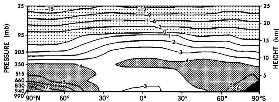
Fig. 14. Latitude height distribution of the zonal mean difference in annual mean temperature (degrees Kelvin) of the model atmosphere between the 4 \times CO_2 and 1 \times CO_2 experiment.
