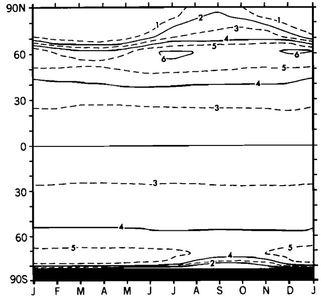
Fig. 18. The latitude-time distribution of the difference in zonal mean surface water temperature (degree Celsius) of the mixed layer model ocean between the 4 × CO 2 and 1 × CO 2 experiments.
