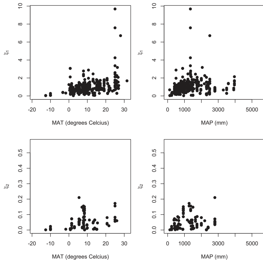
Figure 6. Effects of mean annual temperature MAT ( ^{\circ}\text{C} ) and mean annual precipitation MAP (mm) on decomposition rates from the Soil Respiration Database [Bond-Lamberty and Thomson, 2010b] calculated as \xi_1 (equation (16)) and \xi_2 (equation (17)).
