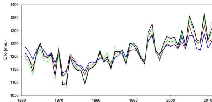
Figure 10. Evolution of the observed regional annual ETo (in black) from 1961 to 2011 and those simulated with each meteorological variable held constant: blue: relative humidity, dark red: maximum temperature, green: minimum temperature, gray: wind speed, dashed: sunshine duration.
