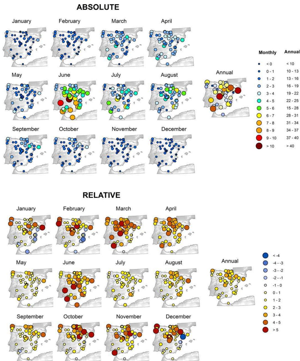
Figure 4. Spatial distribution of monthly and annual changes of ETo at 46 observatories from 1961 to 2011. The change is given in absolute ETo change ( \text{mm decade}^{-1} ) and in relative units ( \% \text{ decade}^{-1} ).
