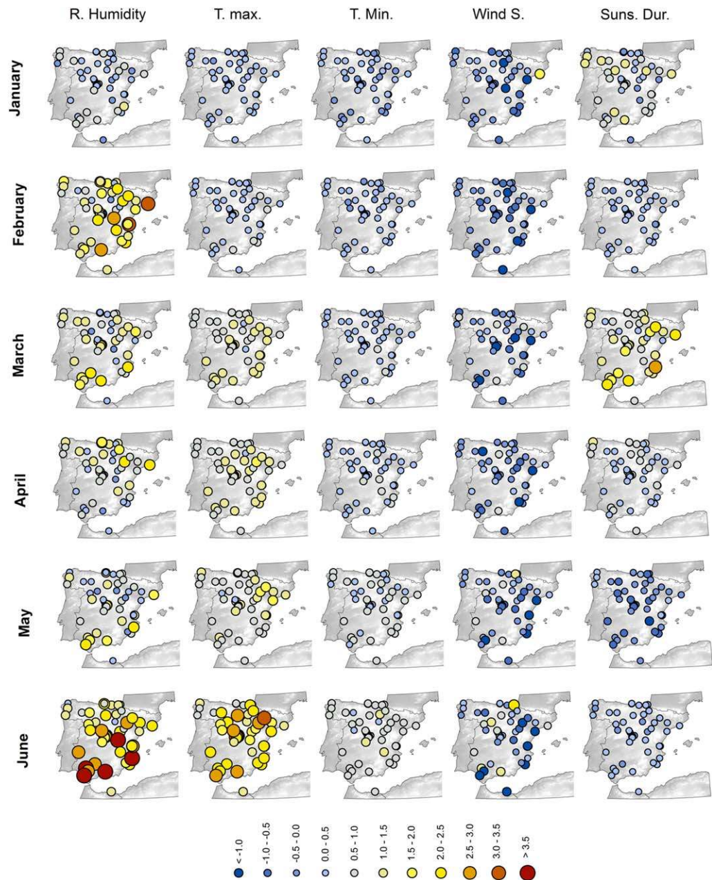
Figure 11. Spatial distribution of the differences between observed monthly and annual magnitude of change in ETo (in mm.) and the simulated monthly and annual magnitudes of change with the meteorological variables held constant. Spatial distribution of the differences between the observed monthly and annual magnitude of change of ETo (in mm.) in the different observatories and the simulated monthly and annual magnitudes of change with the different variables held constant.
