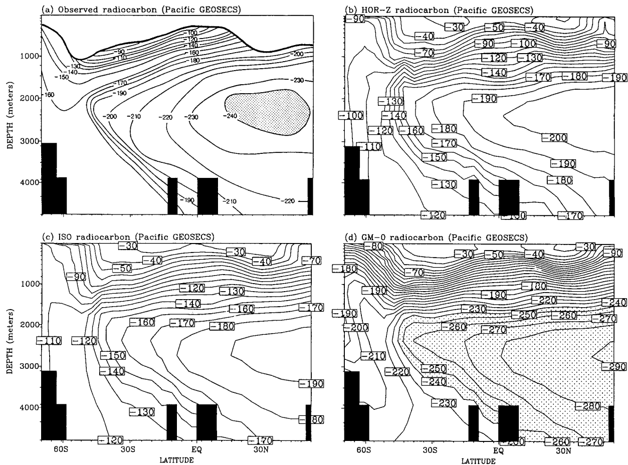
FIG. 16. Observed Pacific Ocean GEOSECS \Delta^{14}\text{C} compared with model runs HOR-Z, ISO, and GM-0. Contour interval is -10\% and stippling indicates waters with \Delta^{14}\text{C} content less than -240\% . In the observed section, no contours are drawn in regions contaminated by bomb-produced ^{14}\text{C} .
