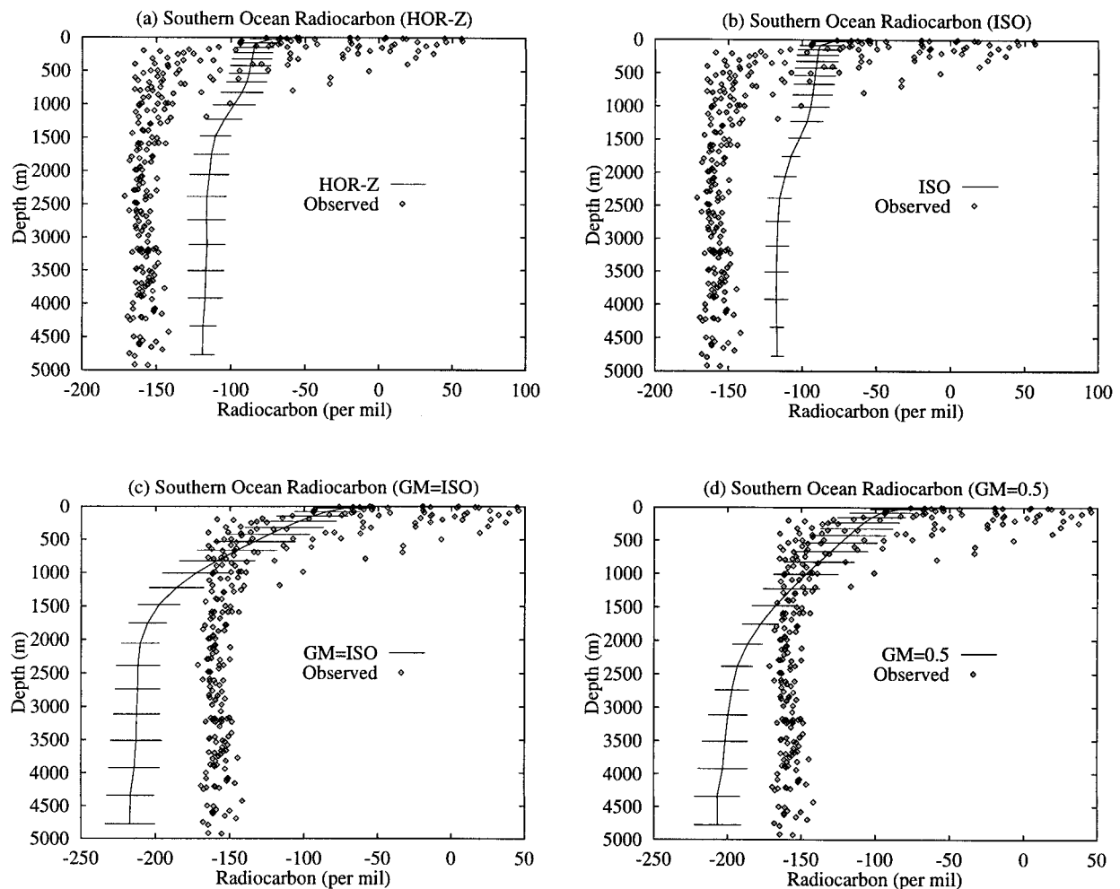
FIG. 13. Model simulations of radiocarbon at the latitude band 55^{\circ} – 70^{\circ} S, shown as a mean profile with standard deviation bars to indicate the spread of ^{14}\text{C} simulated at each depth level. (a) HOR-Z, (b) ISO, (c) GM = ISO, and (d) GM = 0.5. The overlaying scatterplot of GEOSECS ^{14}\text{C} measurements facilitates a direct comparison between modeled and observed ventilation rates. This region corresponds in the real ocean with the location of CDW upwelling and relatively stable surface layer stratification (e.g., Figs. 2a and 3).
