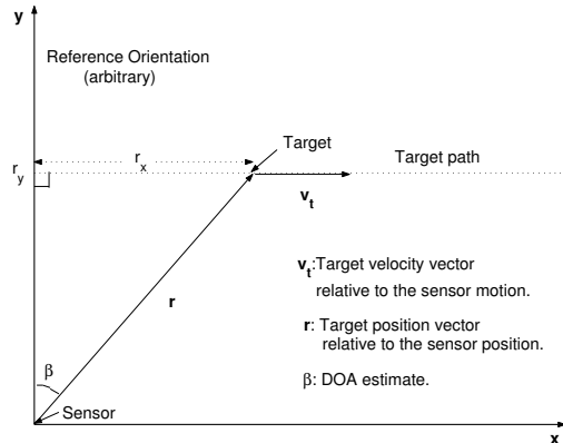
Figure 1: Geometrical configuration of the two dimensional tracking problem, where sensor and target are assumed to lie in the same plane. The target track is assumed to be parallel to the x -direction, and the sensor reference orientation is arbitrarily chosen to be the y -direction. Note that the sensor is situated at the origin.
