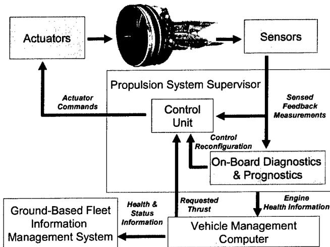
Figure 3. Engine Health Management Architecture
