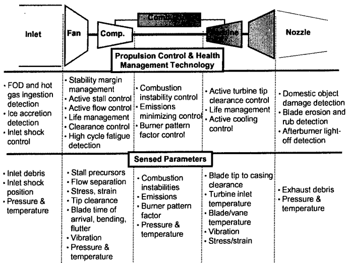
Figure 1. PCHM Technologies and Associated Sensed Parameters
