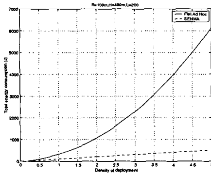
Fig. 2: Energy Efficiency Comparison.
