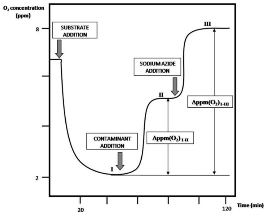
Figure 1. Typical experimental respirometric kinetic curve: analytical parameters are \Delta\text{ppm}(\text{O}_2)_{\text{I-II}} and \Delta\text{ppm}(\text{O}_2)_{\text{I-III}} , where \Delta\text{ppm}(\text{O}_2)_{\text{I-II}} is the variation of \text{O}_2 consumption between steady-state I and II and \Delta\text{ppm}(\text{O}_2)_{\text{I-III}} is the variation of \text{O}_2 consumption between steady-state I and III .
