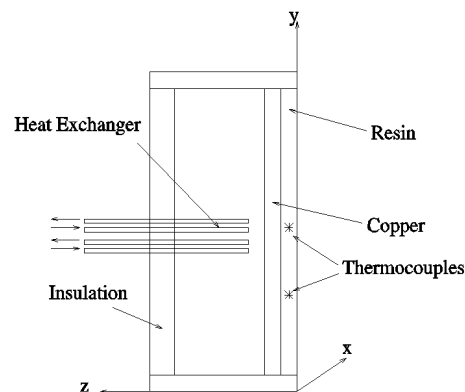
Figure 1. Profile of the active plate.
