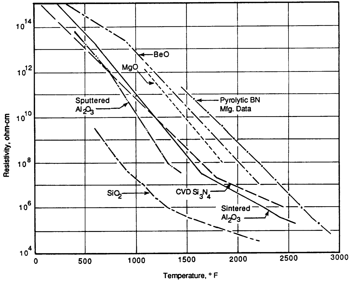
Figure 4. Resistivity Versus Temperature - High Temperature Insulators. Data is from References 2-23 through 2-32.
