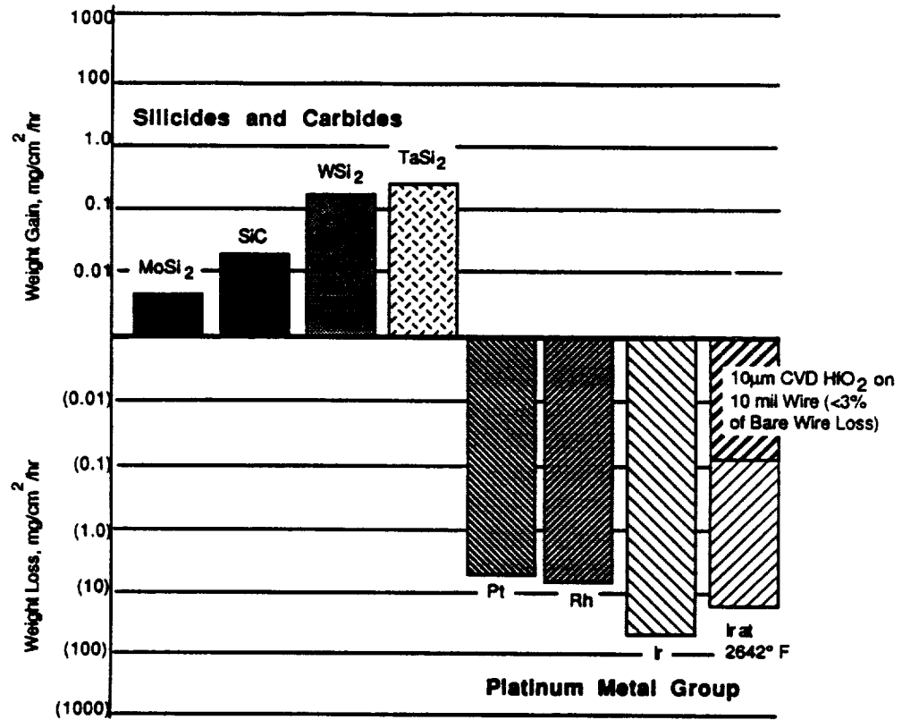
Figure 1. Weight Gain (Loss) Due to Oxidation for Candidate Conducting Materials at 3000 °F in Air.
