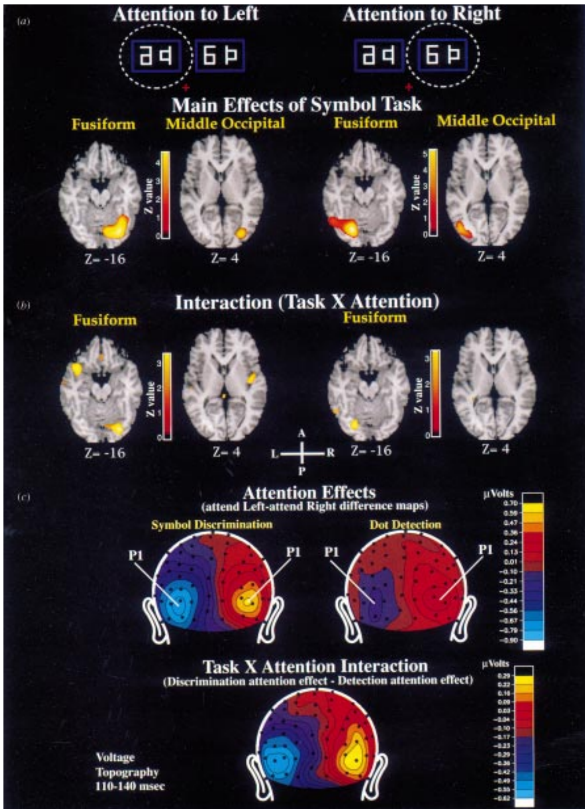
Figure 6. (a) Top row shows examples of bilateral symbols used as stimuli in the study by Mangun et al. (1997). In different runs subjects attended to the right or left side of the displays, which were presented in rapid, randomized order. Brain sections show that attention to the left-field stimuli produced PET activations in the right fusiform and middle occipital gyri, while attention to the right produced corresponding activations in the left hemisphere. Note that left side of the images corresponds to left side of brain. (b) Visual cortex activations were greater for the symbol discrimination task than for a simpler dot detection task only in the contralateral fusiform gyrus. (c) Topographical voltage maps of the attention effect on the P1 component (110–140 ms latency) elicited by the bilateral stimuli. Maps represent P1 voltage distributions in attend left minus attend right conditions. Lower head shows that the P1 attention effect was greater for attend-symbol than for attend-dot conditions, as was the fusiform gyrus activation shown in b .
