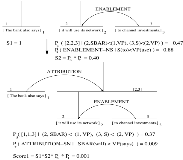
Figure 5: Bottom-up discourse parsing.
