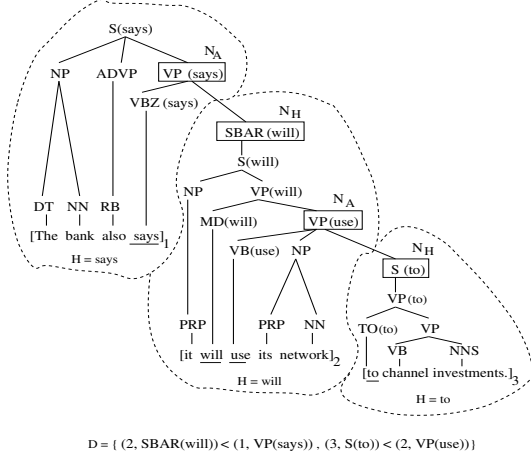
Figure 4: Dominance set extracted from a DS-LST.
